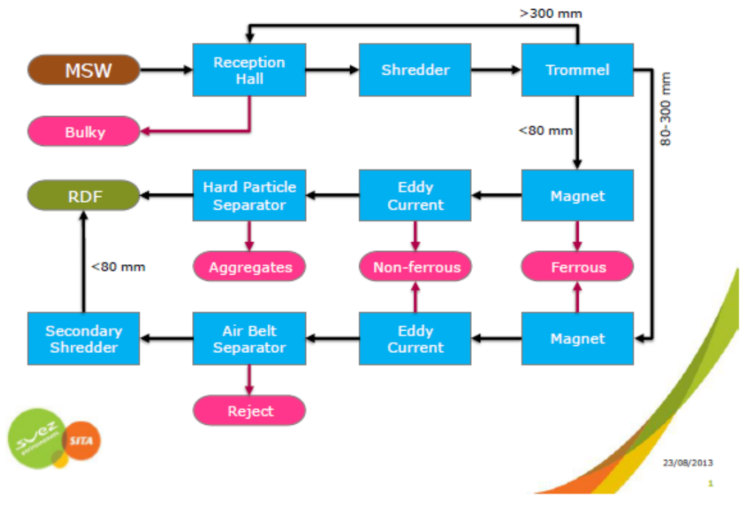
Figure 1: Gasification pre-treatment system flow diagram
