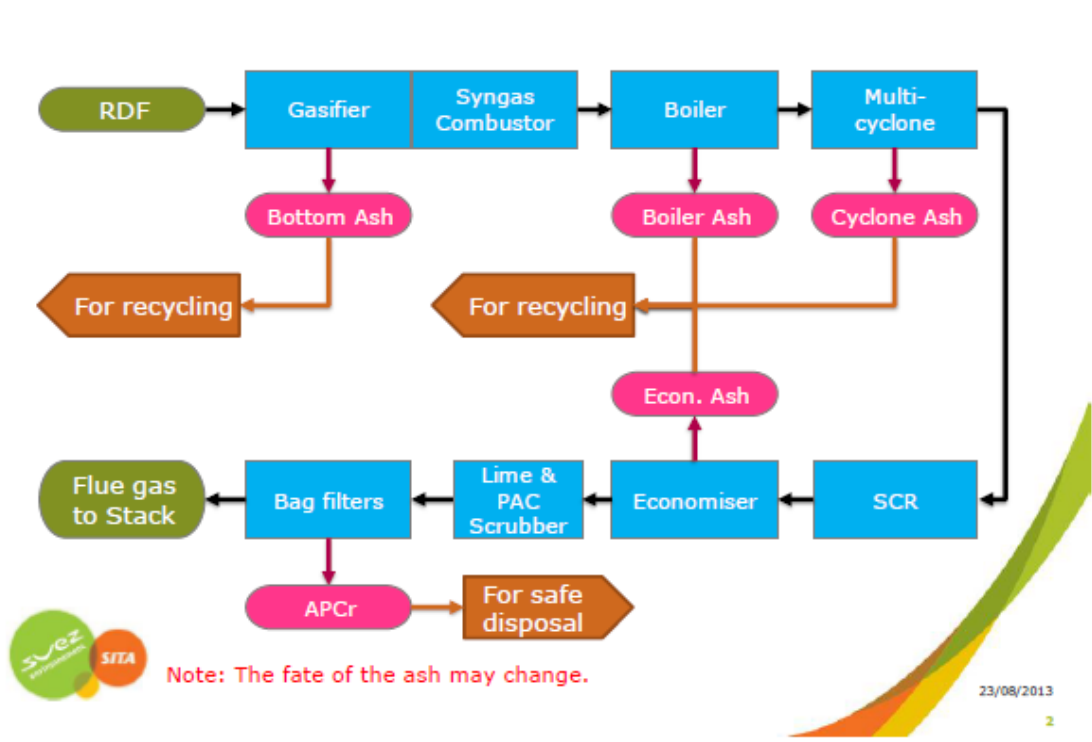
Figure 2: Gasification system flow diagram
