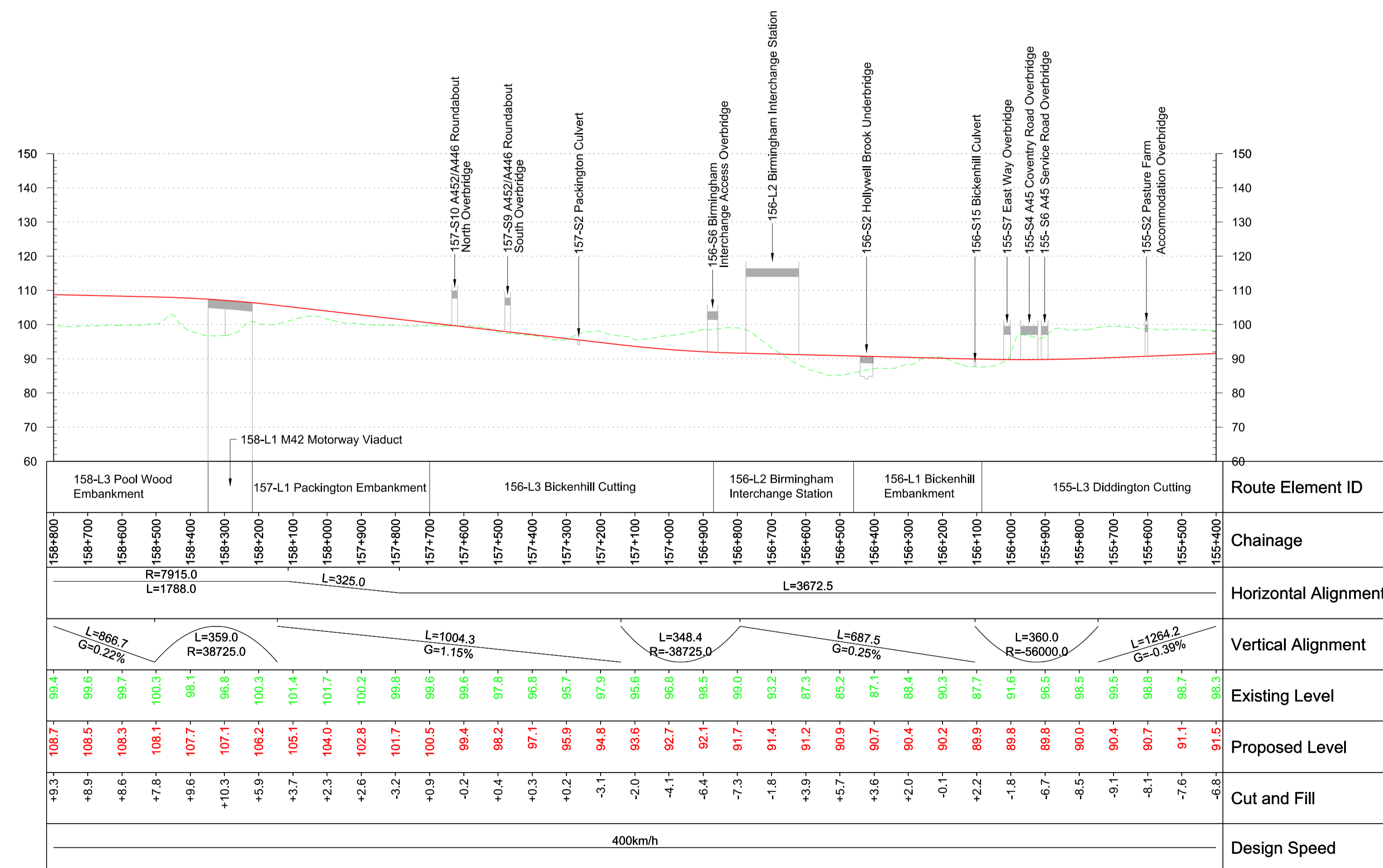
Profile Scale H 1:10000 V 1:1000
