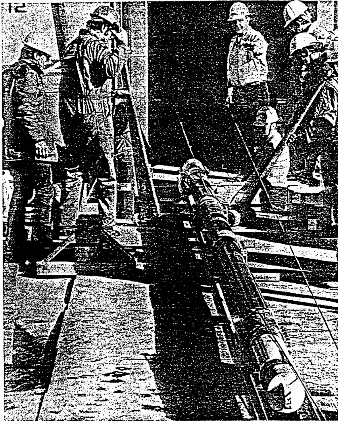
ONE OF THREE 30-kiloton explosives, 30 ft. long and 7 in. in diameter, used for simultaneous detonation in Rio Blanco gas stimulation experiment. Shot went off without a hitch, with almost no seismic effect and no radiation release. Story on p. 7.
