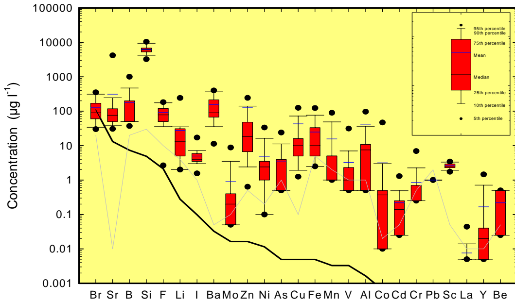
Figure 5.4 Boxplot showing the range of minor and trace element concentrations in the South Staffordshire and North Worcestershire region. Grey line represents typical detection limits for analyses.
