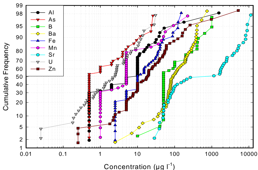
Figure 5.5 Cumulative probability plot of minor and trace elements in the South Staffordshire and North Worcestershire region.
