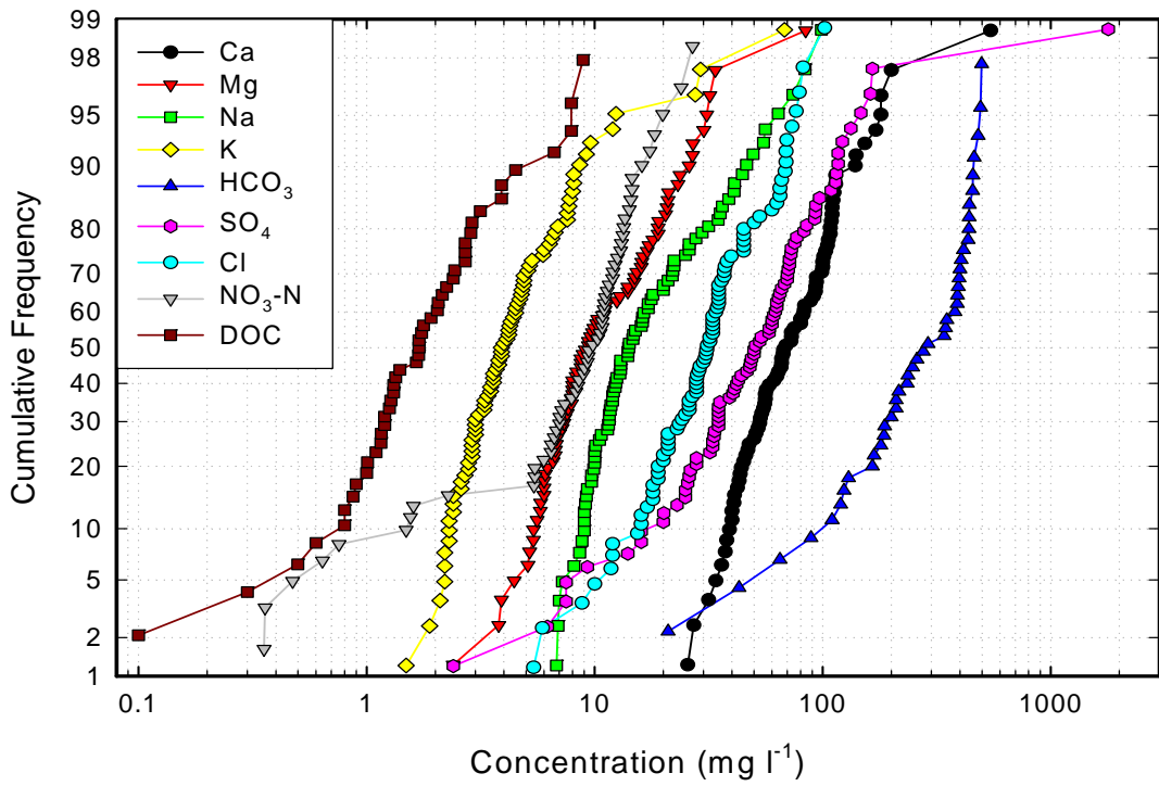
Figure 5.3 Cumulative probability plot of major elements in the South Staffordshire and North Worcestershire region.
