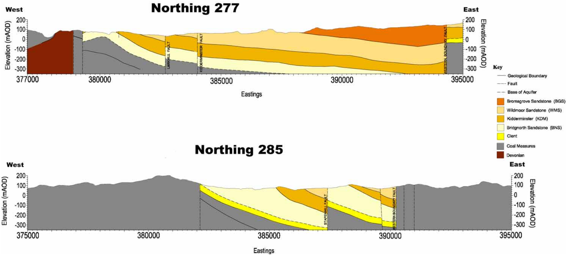
Figure 3.2 East-west cross-sections across the South Staffordshire and North Worcestershire study area (after Entec, 1998). Lines of section are shown on Figure 3.1.
