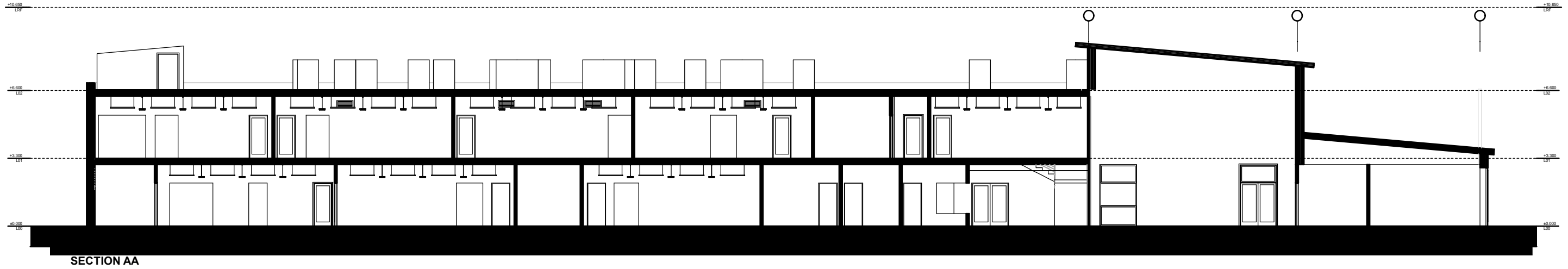
SECTION AA
