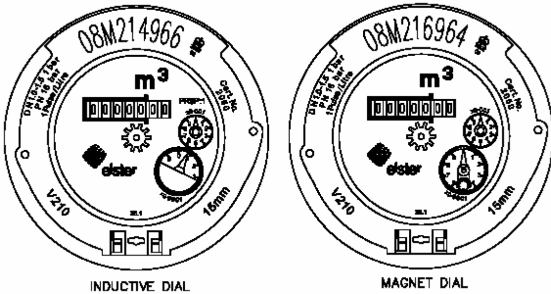
Figure 57 Alternative dial and shroud markings
