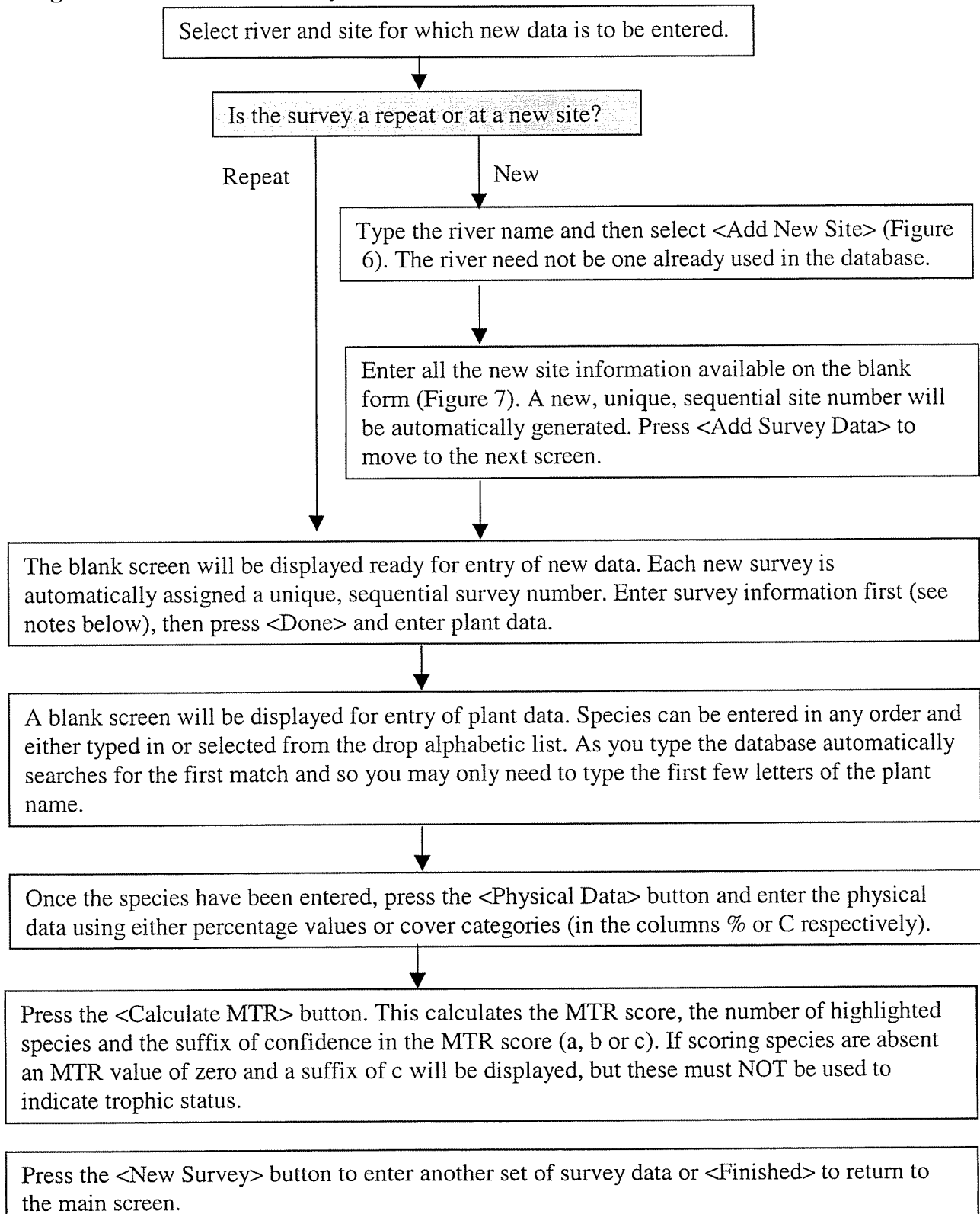
Figure 5. Flow chart for entry of data.
