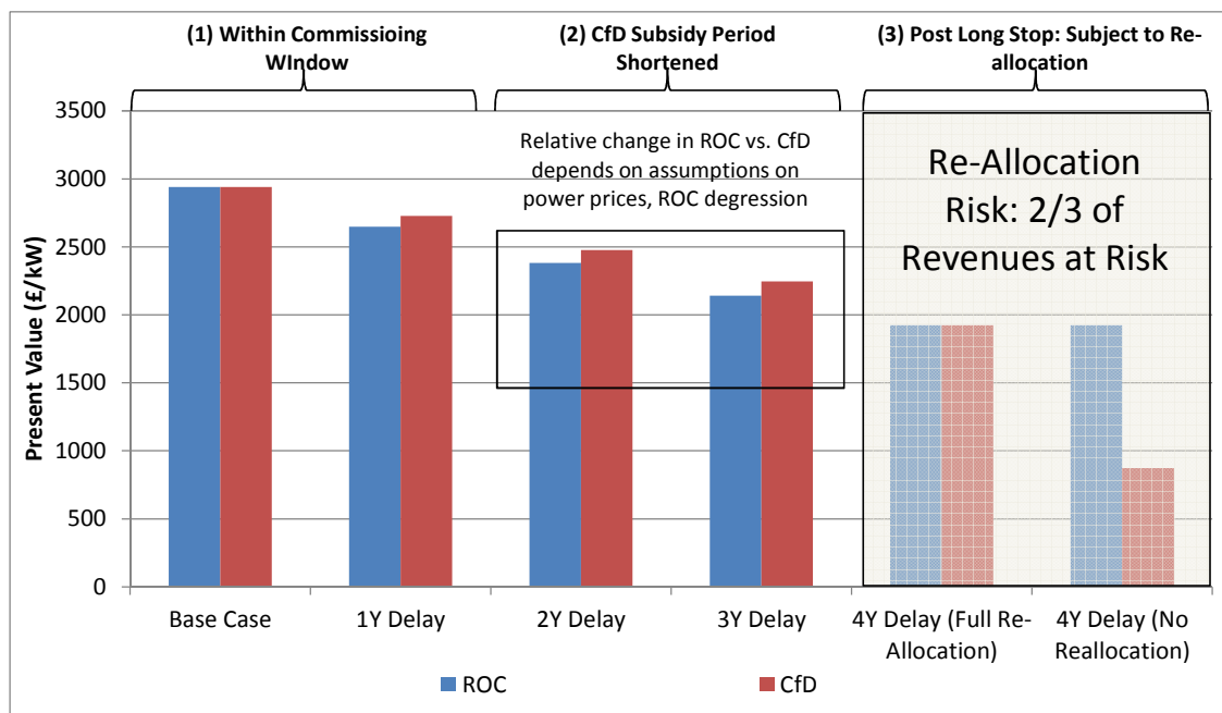
Figure D.14 Effect of Construction Delay for Offshore Wind Asset
