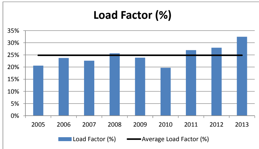
Figure C.2 Load Factor for Onshore Portfolio
