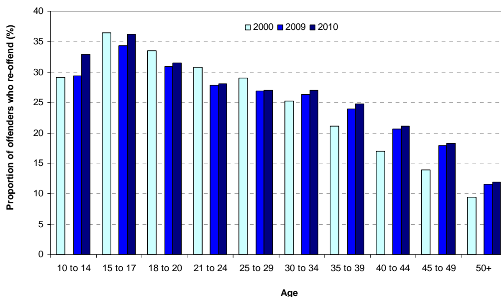
Figure E1: Proportion of offenders who commit a proven re-offence, by age, 2000, 2009 and 2010
