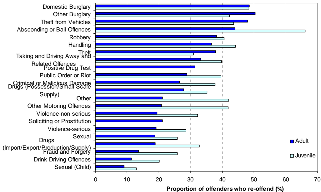
Figure E2: Proportion of adult and juvenile offenders who commit a proven re-offence, by index offence, 2010
