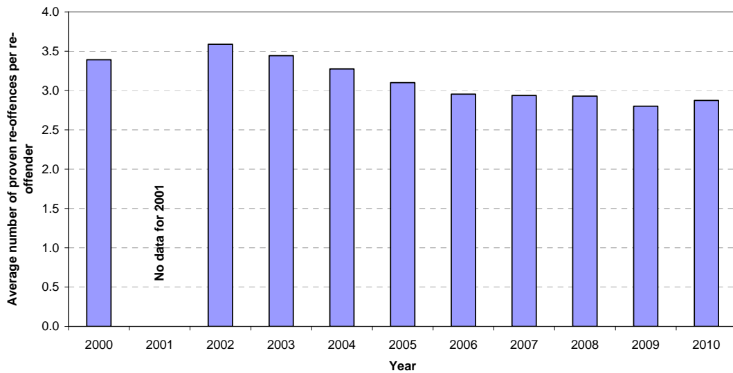
Figure E4: Average number of proven re-offences per adult re-offender, 2000, 2002 to 2010 1
