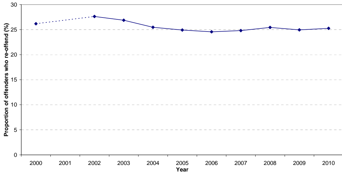
Figure E3: Proportion of adult offenders who commit a proven re-offence, 2000, 2002 to 2010 1
