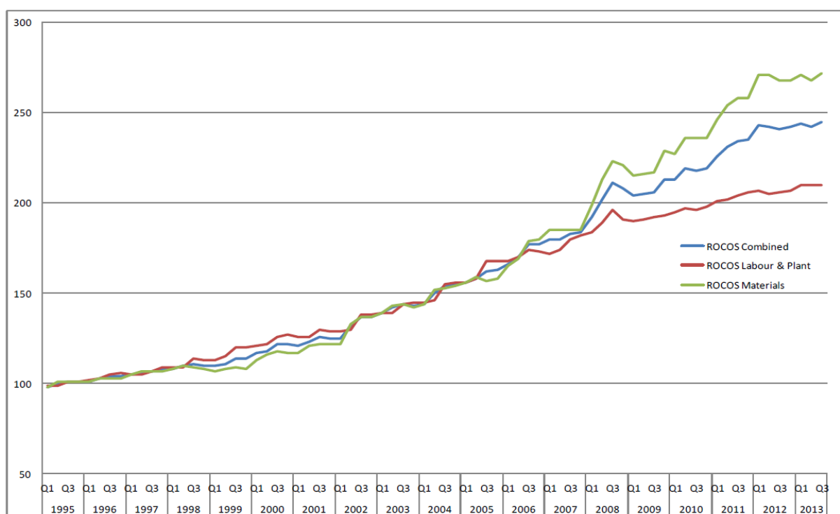
Figure 2: Trends in Road Input Cost Indices ROCOS (1995=100)
