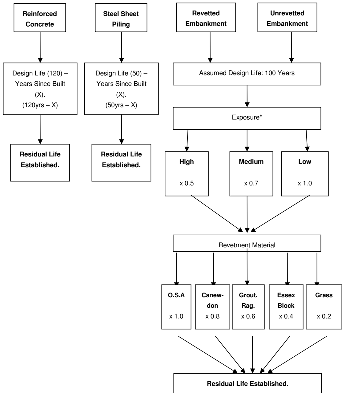
Figure 3-2 Determination of Estimated Unmaintained Life
