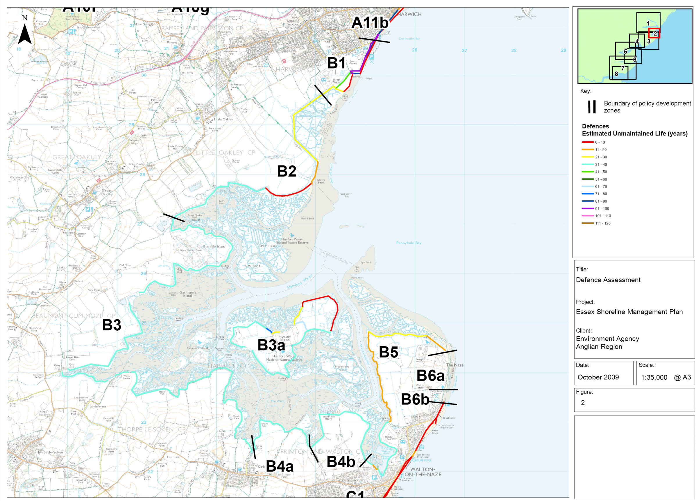
Figure 3-5 Estimated Unmaintained Life of Defences in Hamford Water
