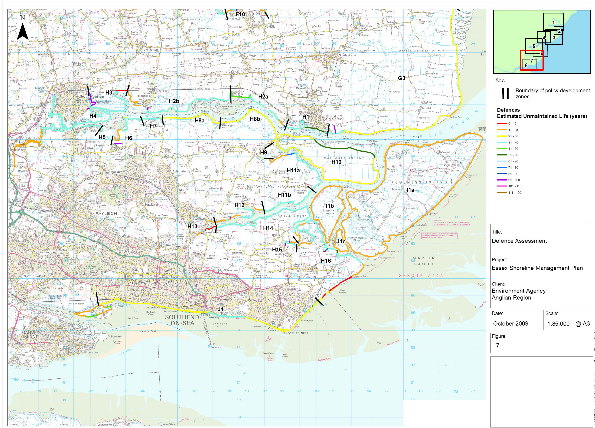
Figure 3-10 Estimated Unmaintained Life of Defences in the Crouch and Roach, Foulness and Southend
