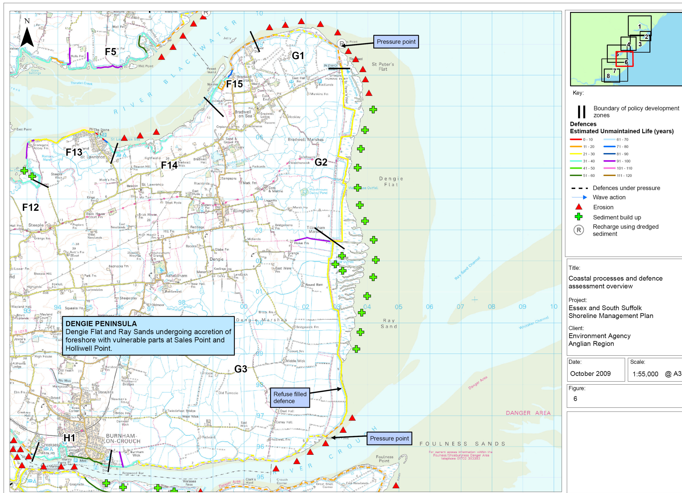
Figure 4-6 Coastal processes and defence assessment overview - Dengie peninsula
