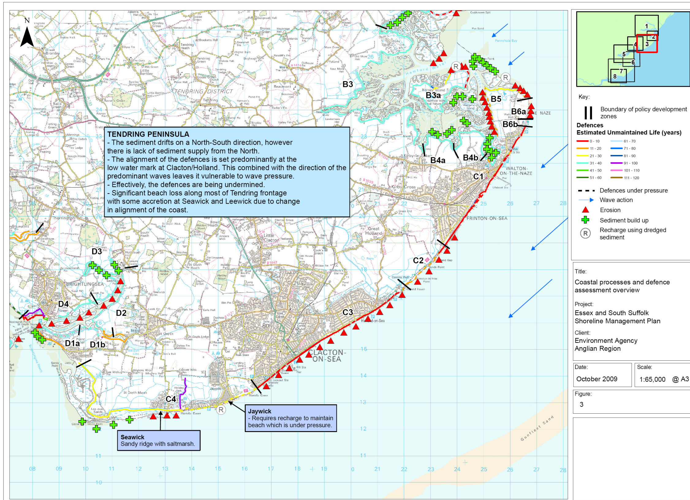
Figure 4-3 Coastal processes and defence assessment overview - Tendring
