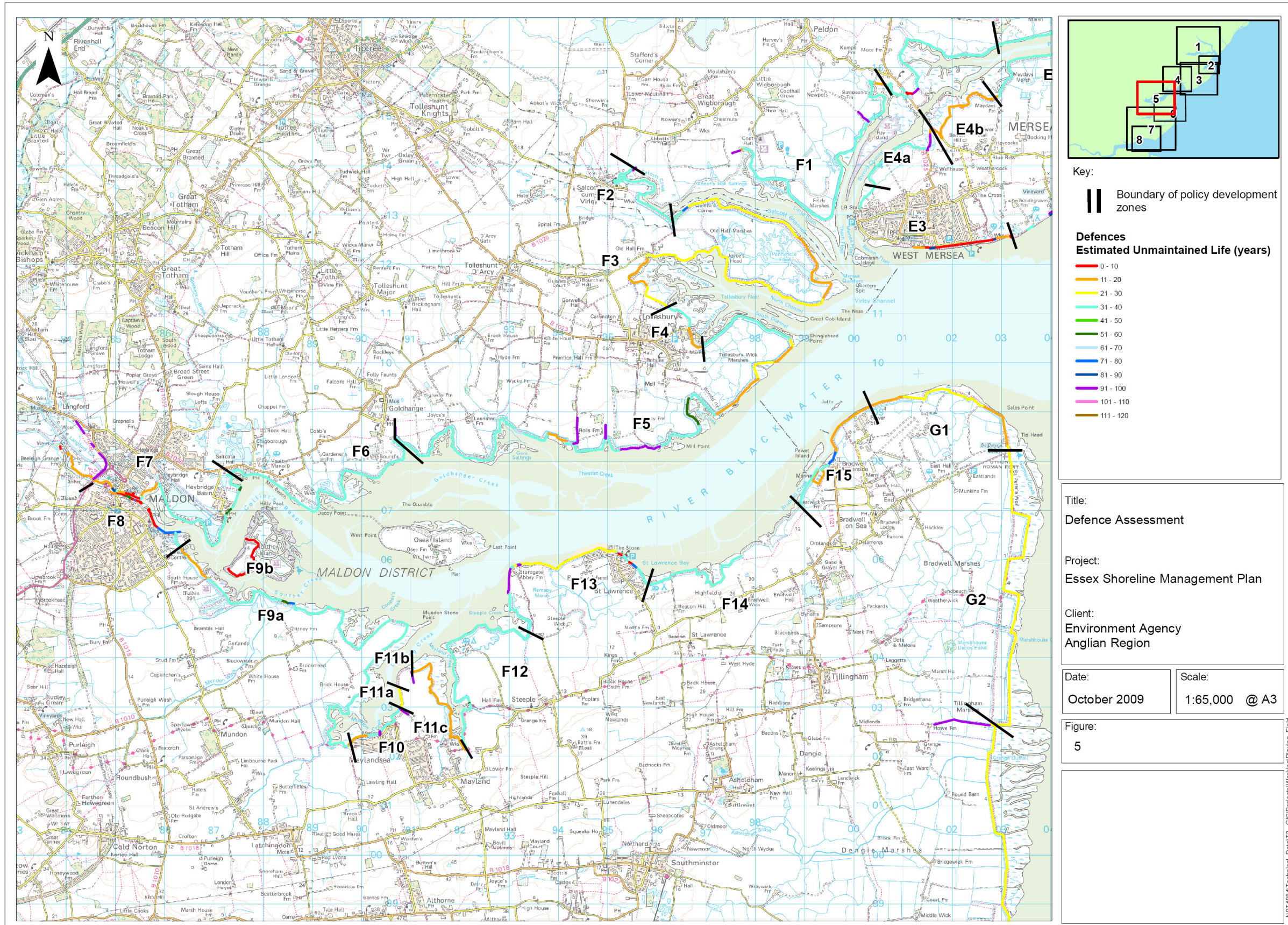
Figure 3-8 Estimated Unexpired Life of Defences in the Blackwater Estuary
