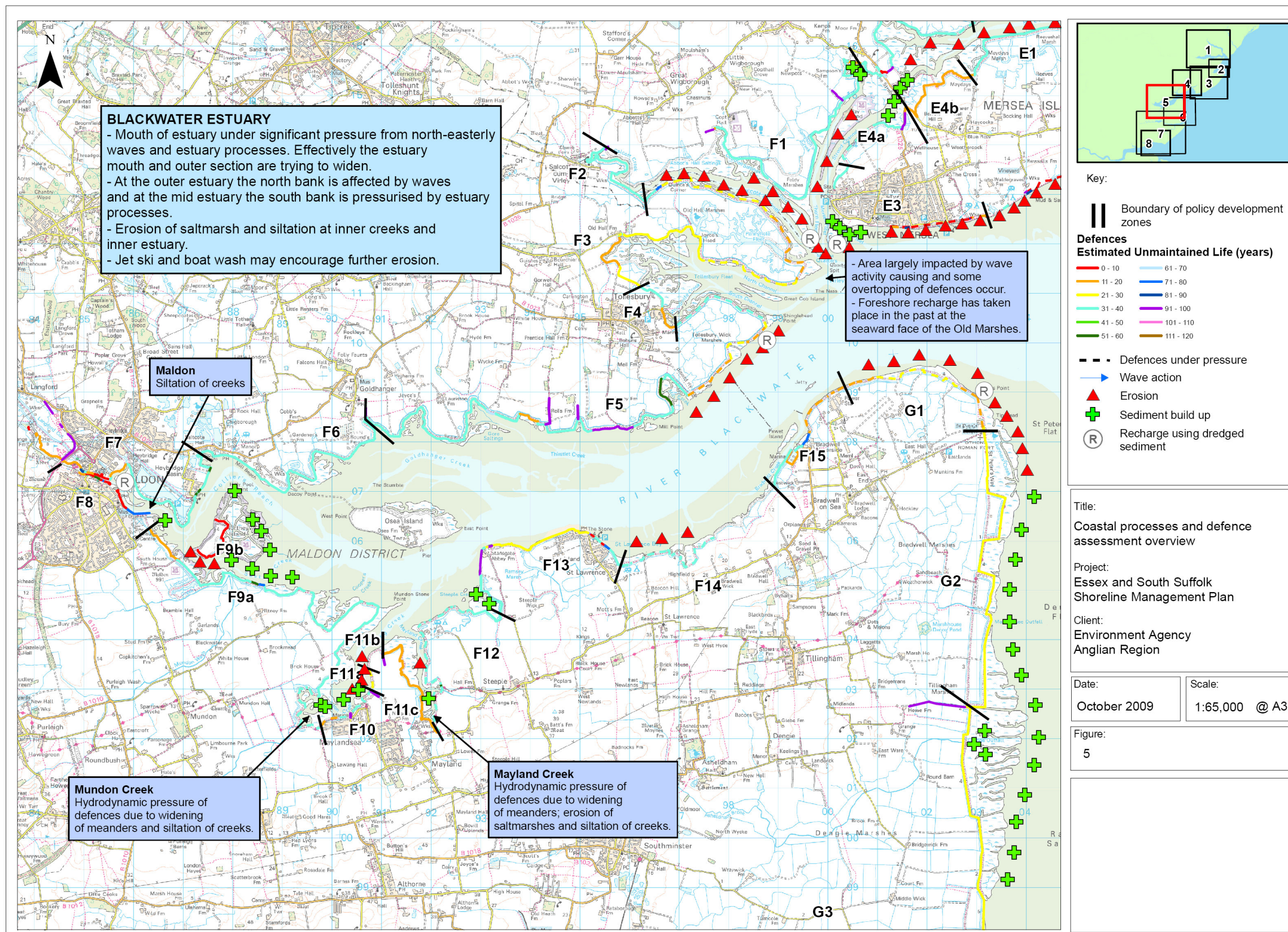
Figure 4-5 Coastal processes and defence assessment overview - Blackwater Estuary
