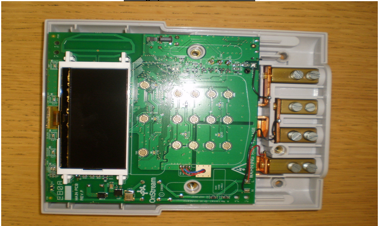
Photograph of meter Internal View 3
