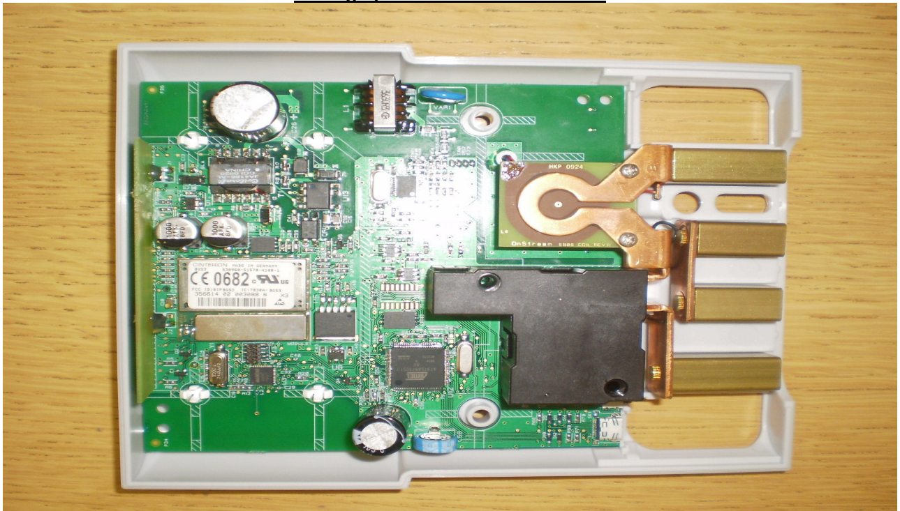
Photograph of meter Internal View 3
