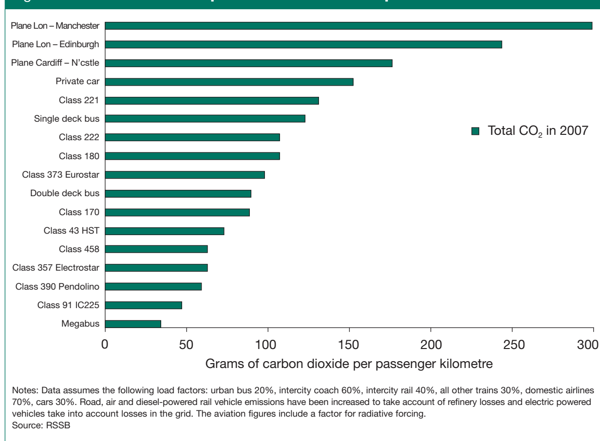
Figure 11.1: Relative carbon performance of rail compared to other modes 9
