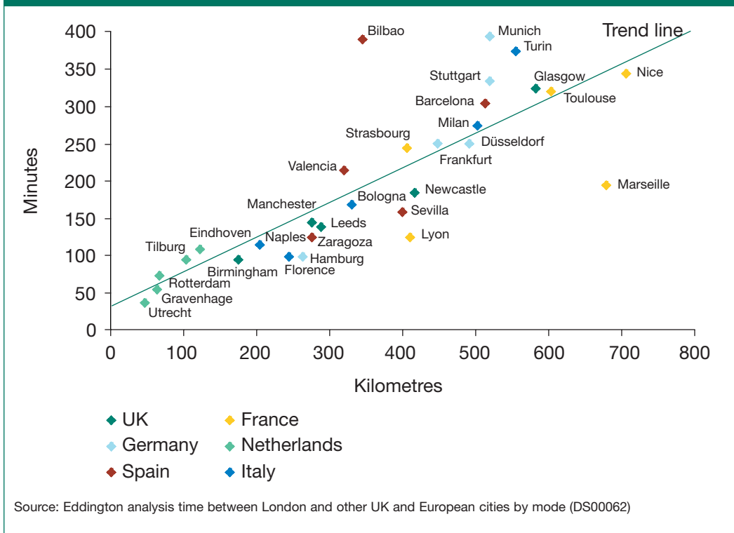
Figure 6.4: Door-to-door journey time versus distance for rail journeys from capital city by country
