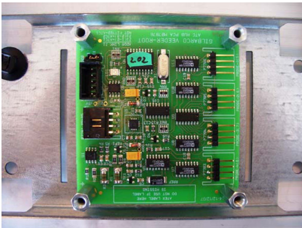
Figure 39 ATC Hub Board
