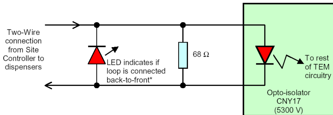
Figure 38 TEM Block Diagram
