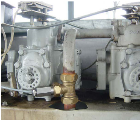
30 Typical installation of temperature sensor
