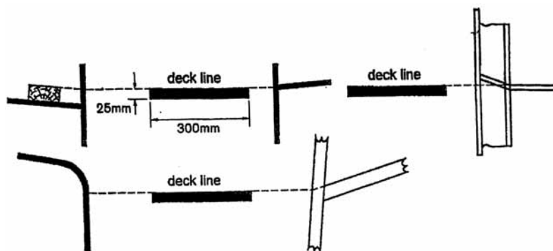
Figure 4.1 Deck line
