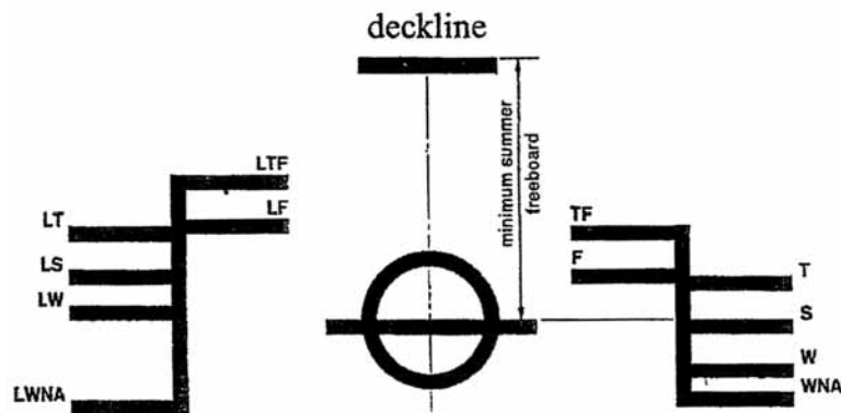
Figure 6.1 Load line mark and lines to be used with this mark
