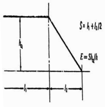
Figure 34.1 Height of superstructure equal to or smaller than the standard height
