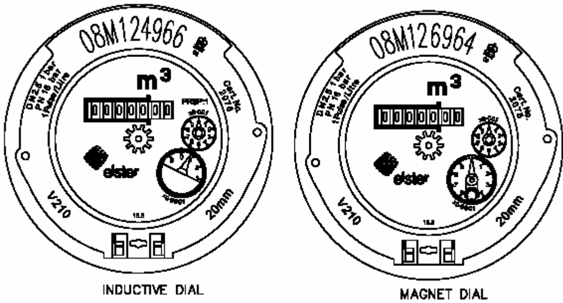
Figure 47 Alternative dial and shroud markings
