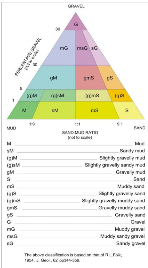
Figure 38 Seabed-sediment classification scheme.
