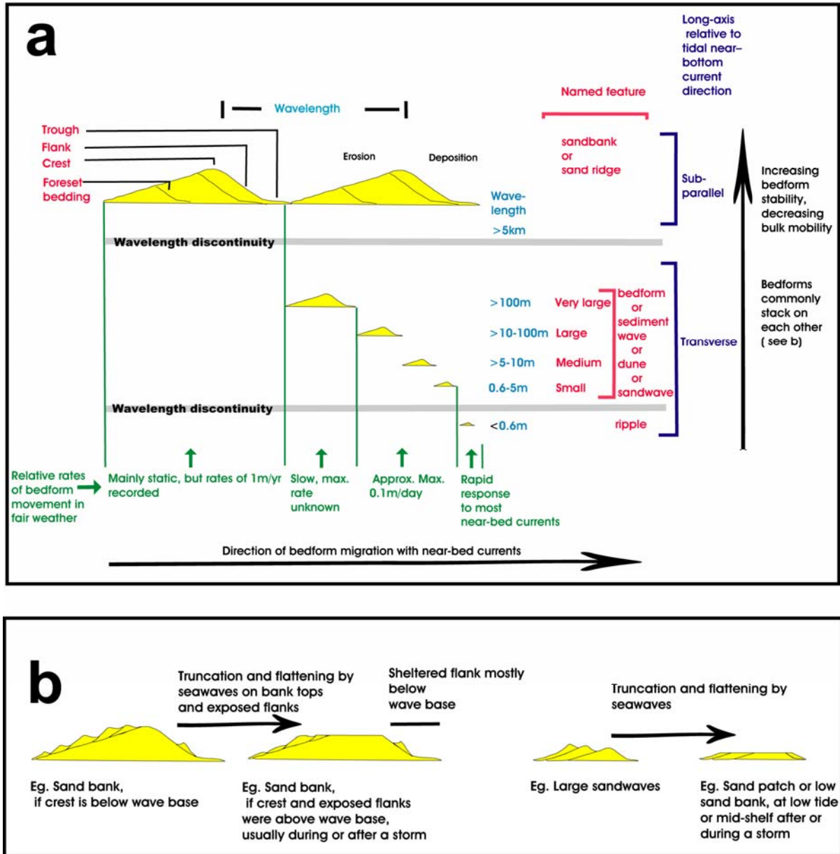
Figure 39 a. Generalised geometries and characteristics of sandwaves and tidal sandbanks related to tidal currents b. observed effects of wave-driven processes on tidal sandbanks and sandwaves
