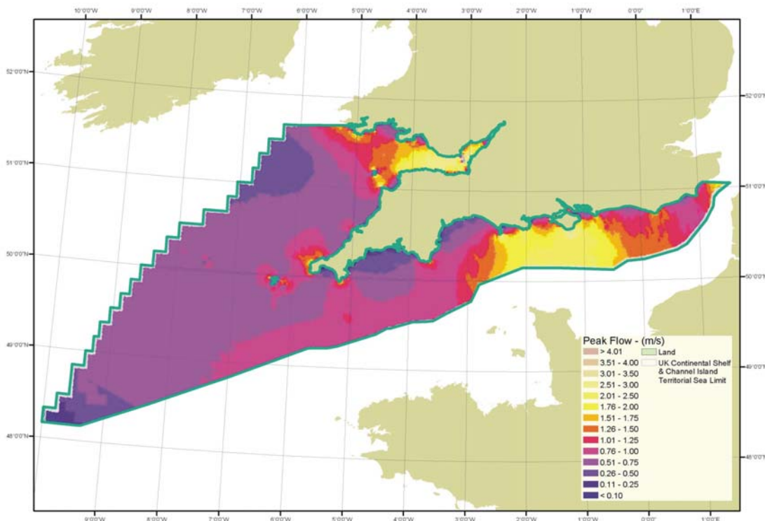
Figure 6. Peak flow for a mean Spring Tide (From DTI Atlas of UK Marine Renewable Energy Resources).
