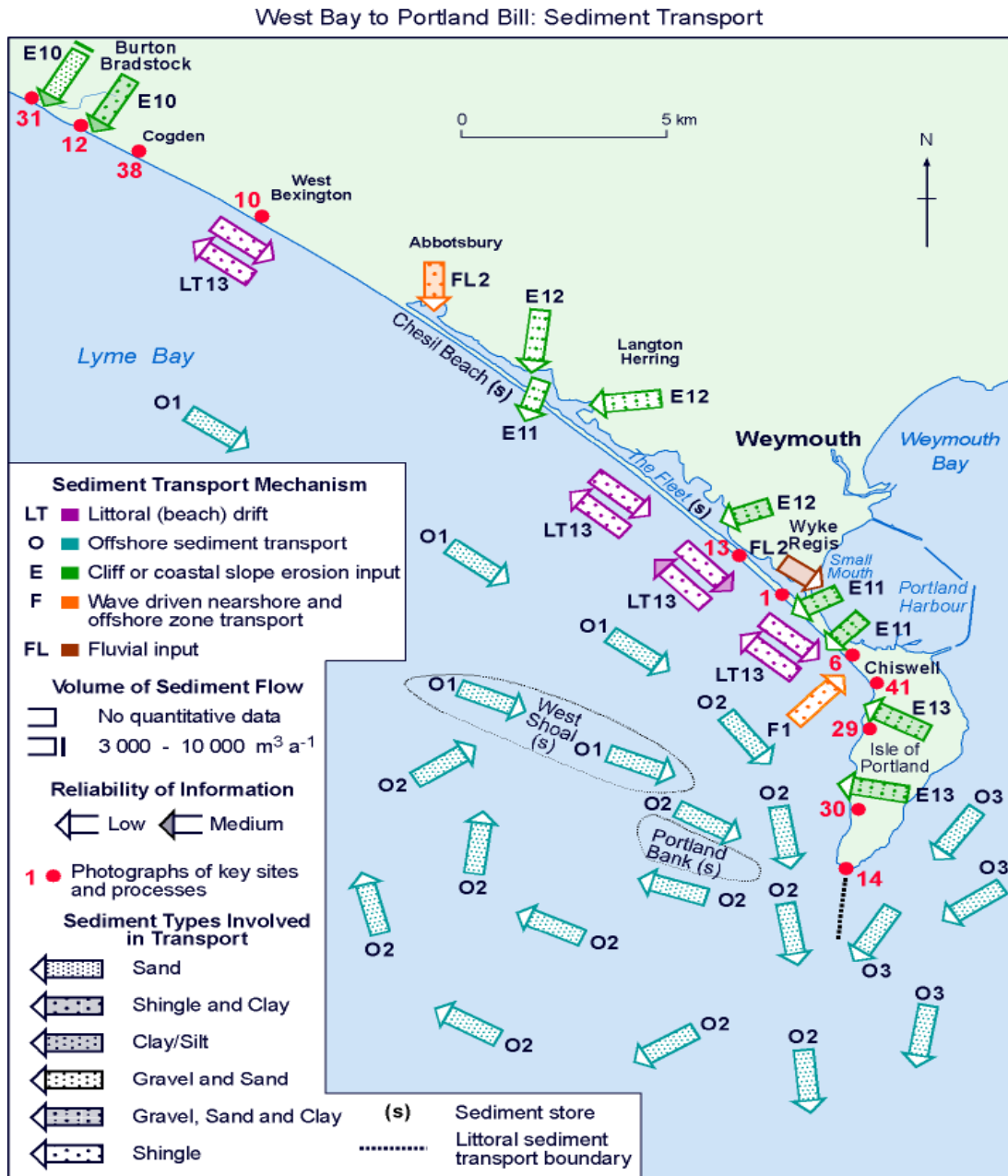
Figure 24. Near- and offshore sediment transport pathways, West Bay to Portland Bill (Bray et al. 2004).
