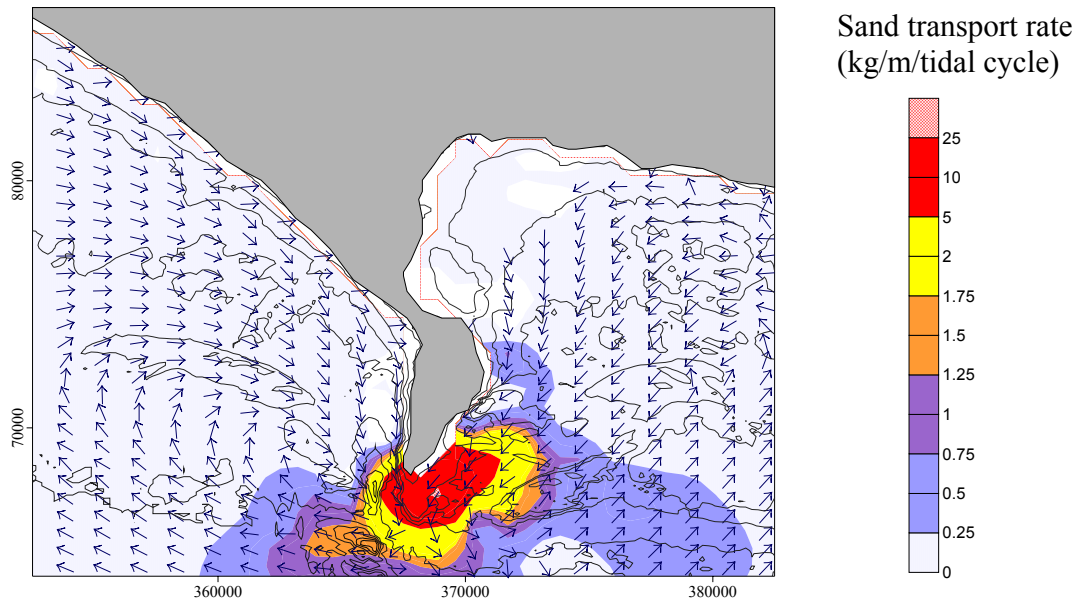
Figure 25. Net total load sand transport rates under the action of waves and currents (Bastos and Collins, 2002).
