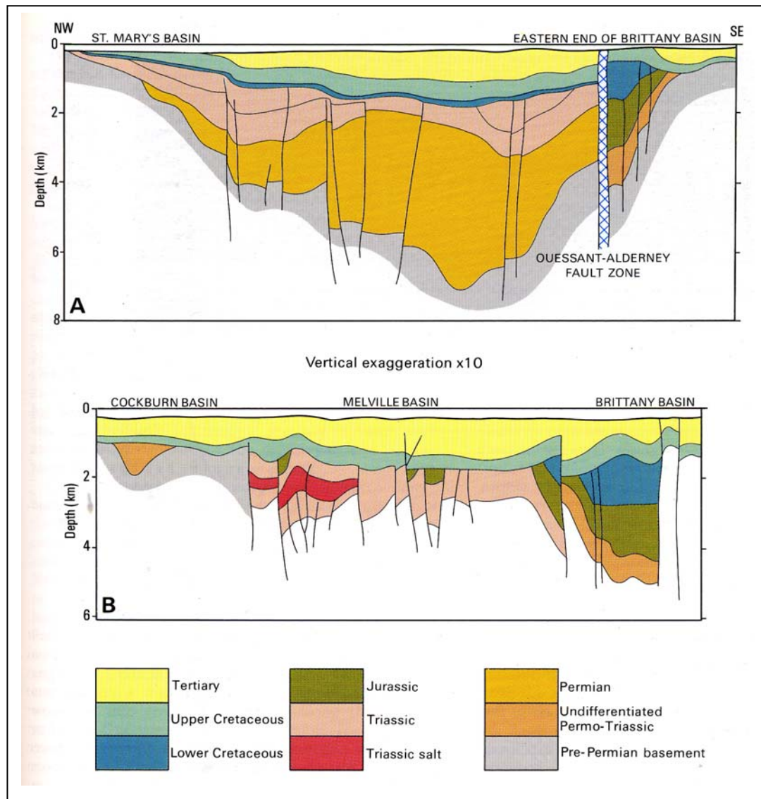
Figure 33. Cross section of the Western Approaches Trough (for location see Figure 24) (From Evans, 1990).
