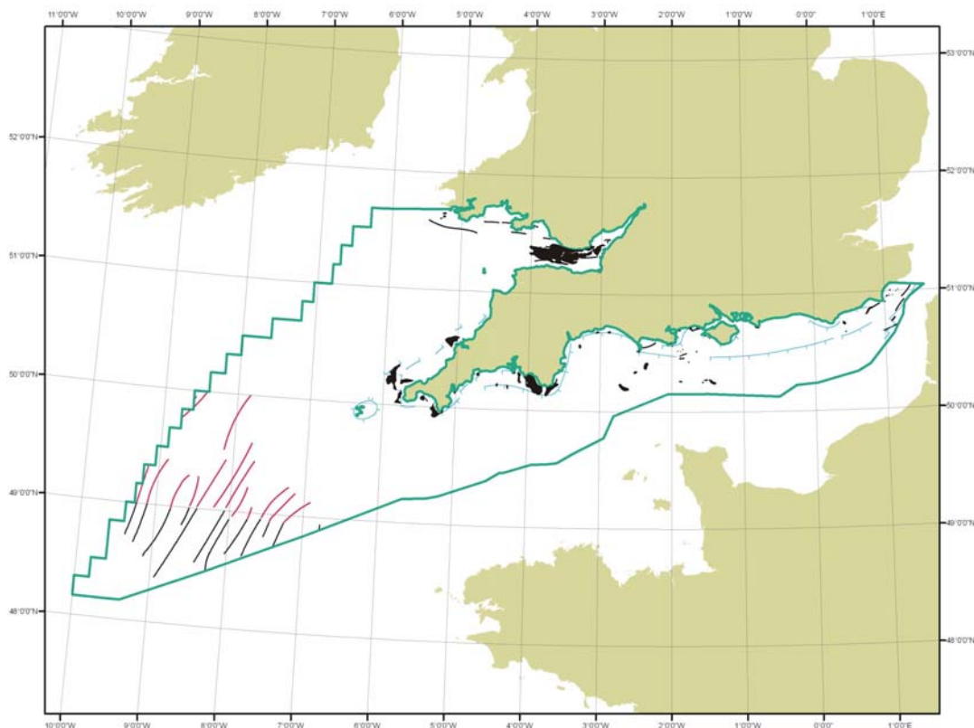
Figure 11. Relict bedforms in SEA8
