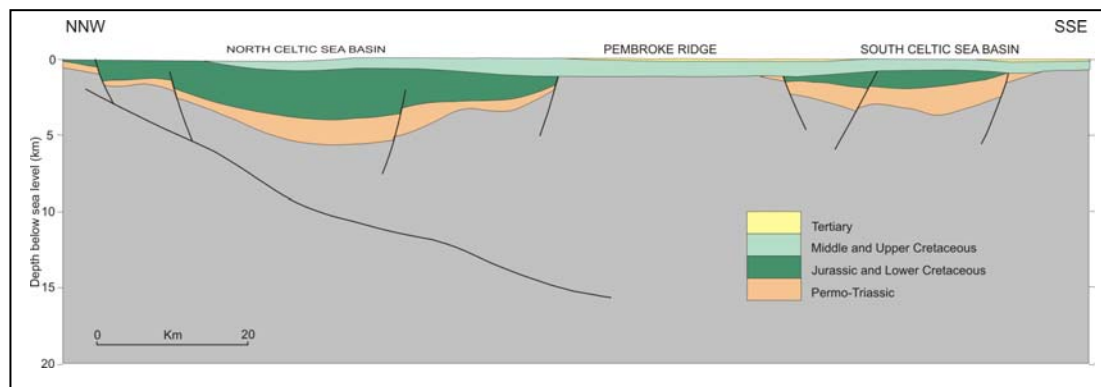
Figure 31. Cross section of the North and South Celtic Sea basins (Location on Figure 24) (From Tappin et al., 1994).
