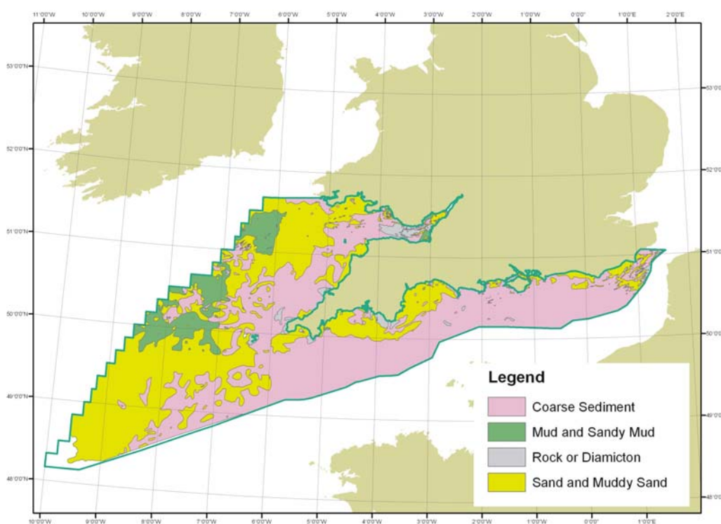
Figure 26. Simplified seabed sediments distribution map of SEA8 area
