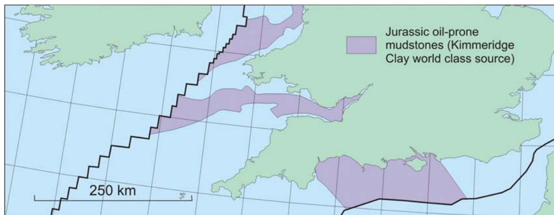
Figure 32. Distribution of Jurassic source rocks in SEA8 area (Derived from DTI, 2004).
