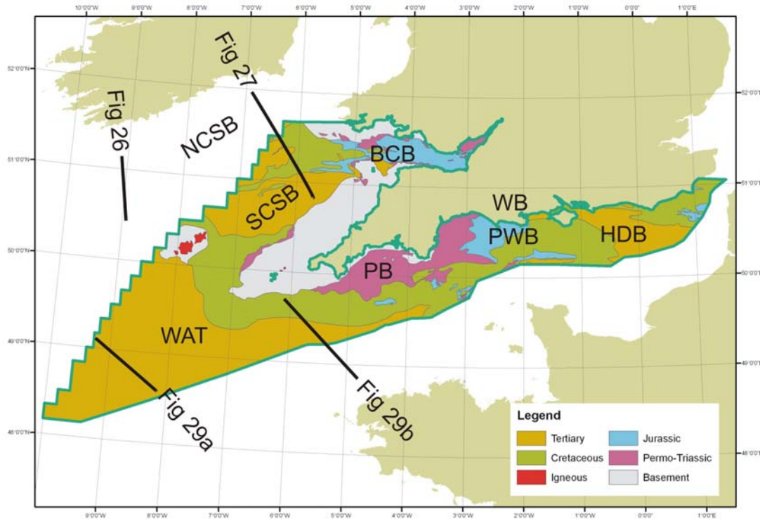
Figure 28. Simplified bedrock geology and main sedimentary Basins in SEA8.
