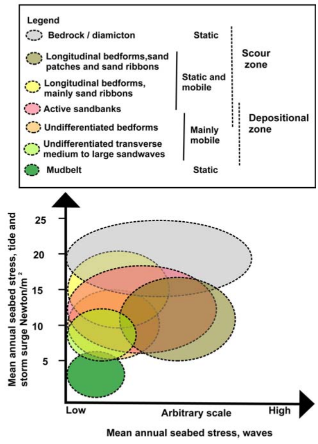
Figure 13. Schematic summary of the observed relationships between mean seabed stress and mobile and static bedforms (From Holmes et al., 2005).
