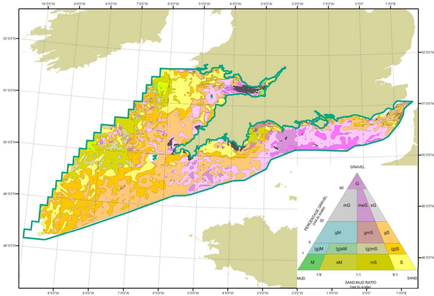
Figure 9. Seabed sediment distribution for SEA8 (For key to sediment type see Figure 37; black regions are exposed bedrock – no sediment.)
