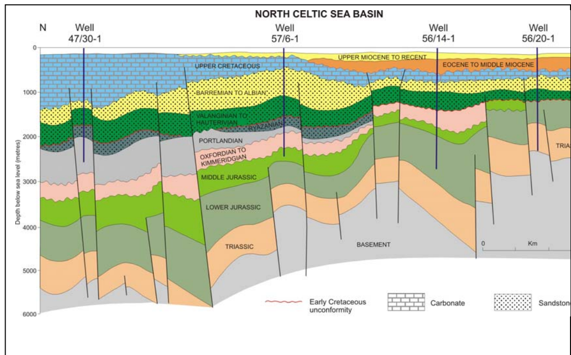
Figure 30. Cross section across the North Celtic Sea Basin (Location on Figure 24) (From Colin et al., 1992).
