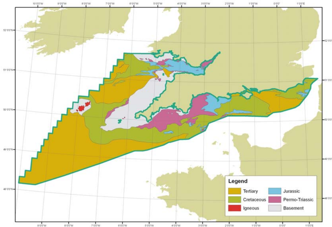
Figure 8. Simplified Bedrock Geology of SEA8
