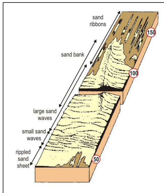
Figure 16. Scheme of bedform zones from a tidal sea where sand is abundant, with corresponding mean spring peak near surface tidal currents in cm/sec (Belderson et al 1982).
