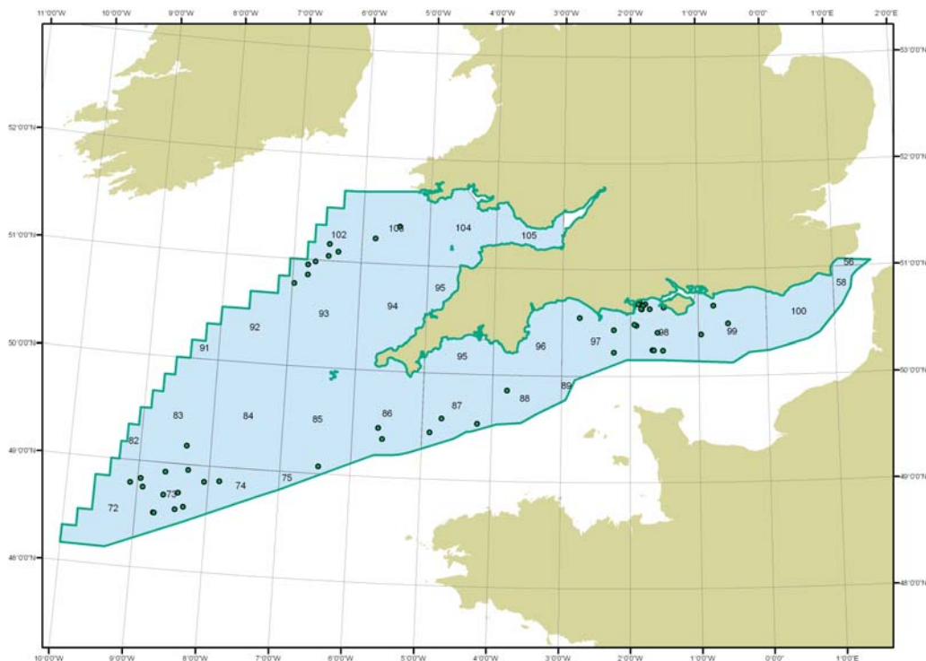
Figure 29. SEA8 Hydrocarbon Quadrants and Commercial Wells (From DTI website).
