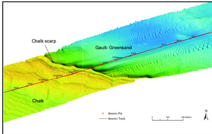
Figure 20 Seabed exposures of a Chalk scarp and underlying Gault-Greensand with a thin sediment cover forming sand waves.
