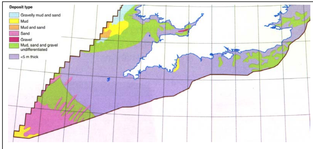
Figure 10. Generalised distribution patterns of sub-seabed sediments.
