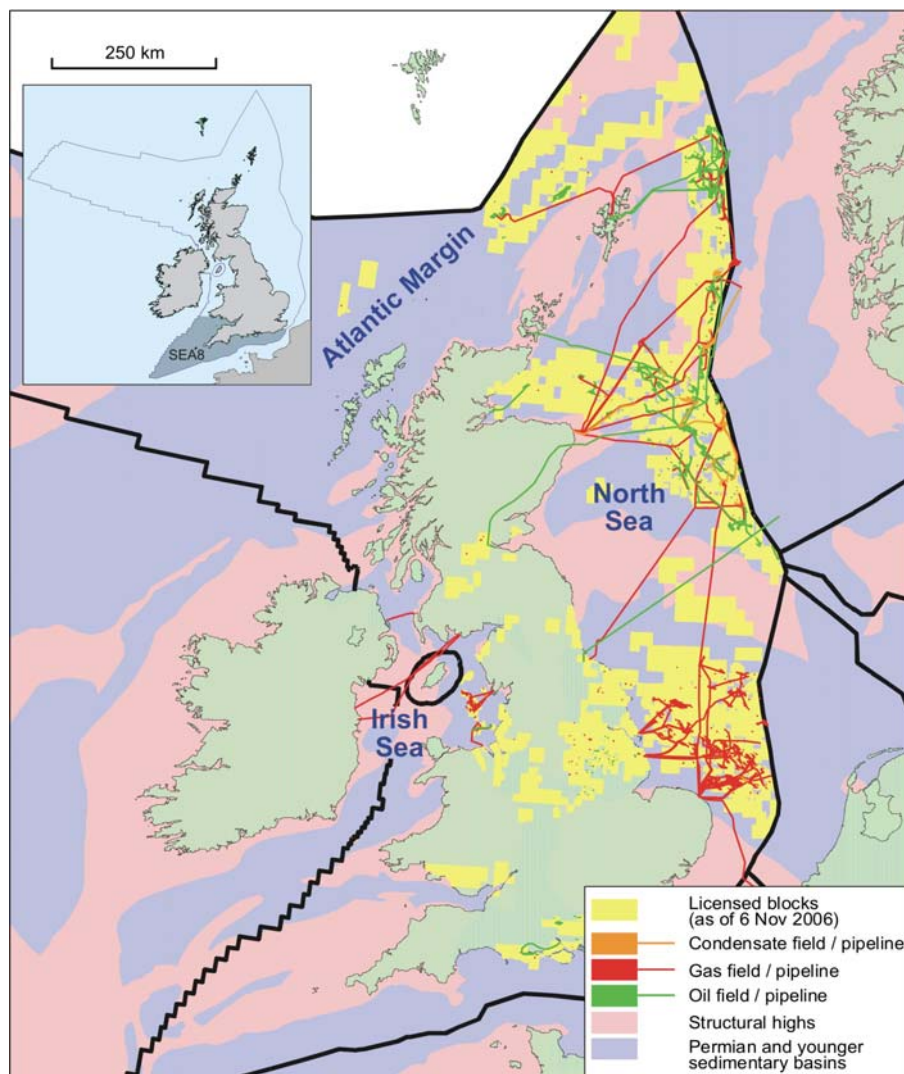
Figure 27 Regional geological setting and hydrocarbons infrastructure (Adapted from DTI 2004).
