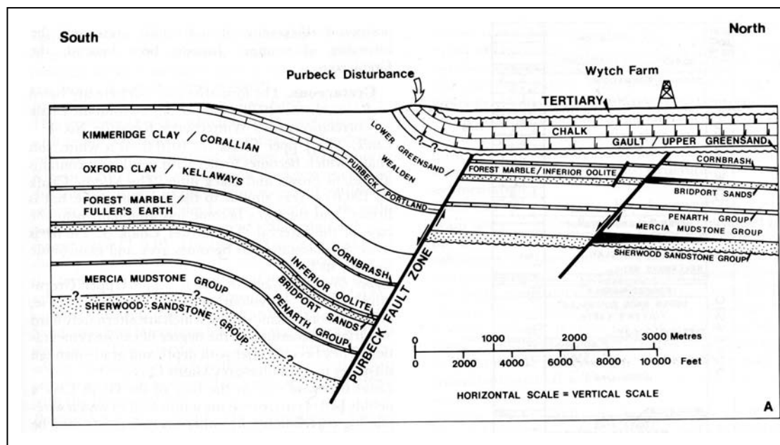
Figure 35. Cross section of the Wytch Farm Oilfield (From Colter and Harvard, 1981).
