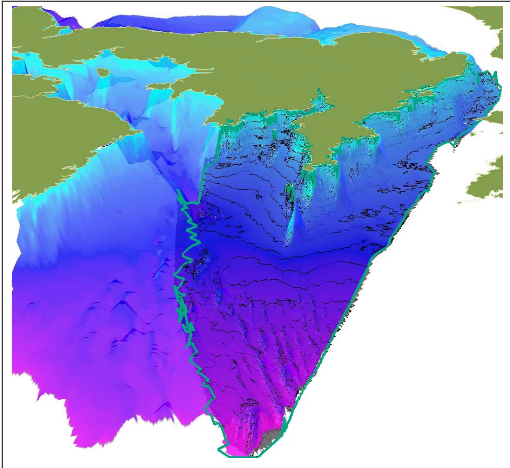
Figure 5. Regional seabed physiography of SEA8 viewed from the southwest
