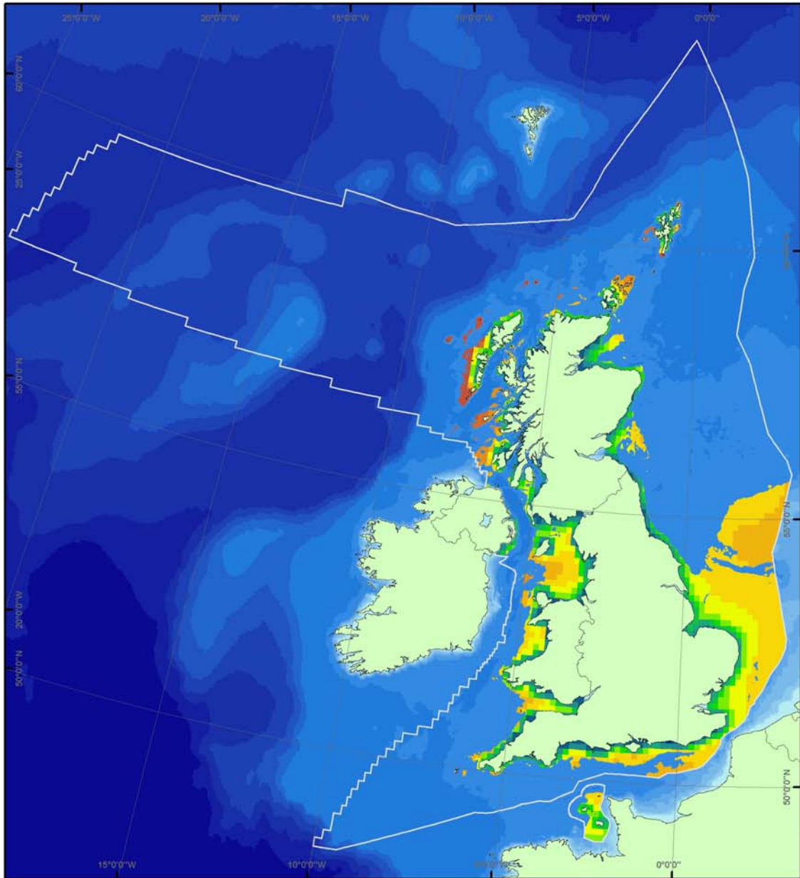
Figure 3 – Annual Mean Wind Power Density in Water Depths of <50 metres
