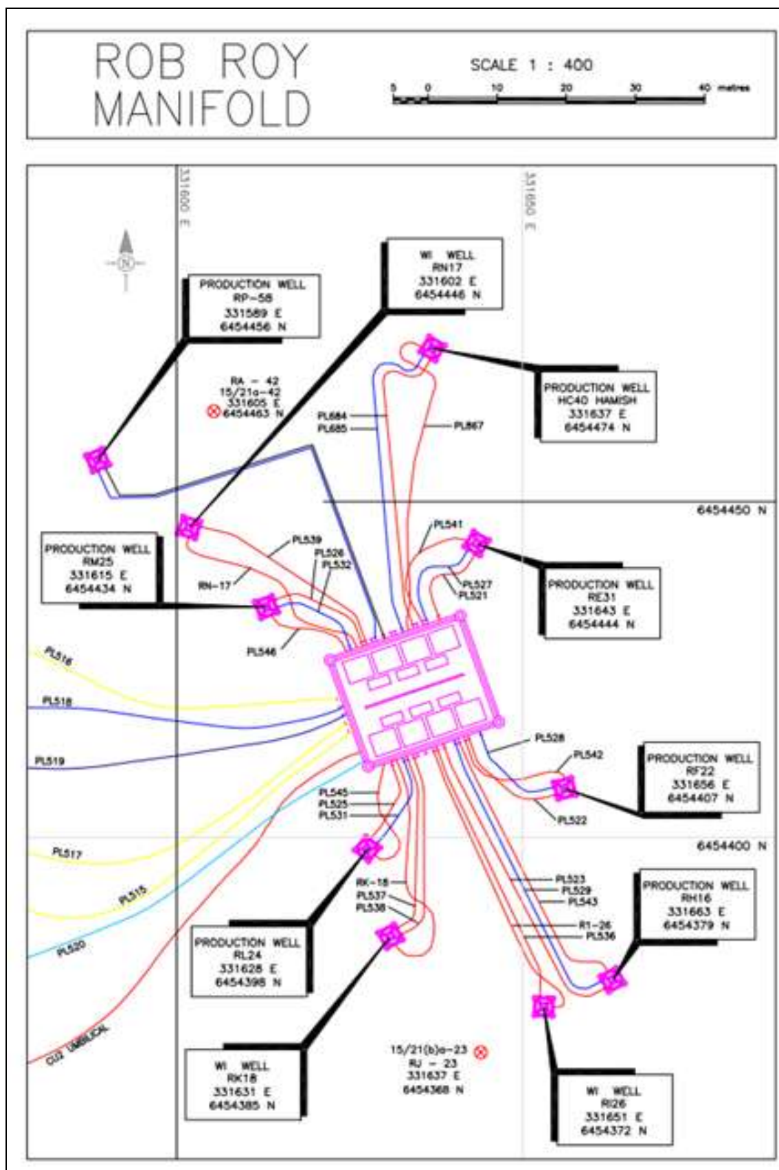
Figure 4.9: The Rob Roy Well Centre Infrastructure
