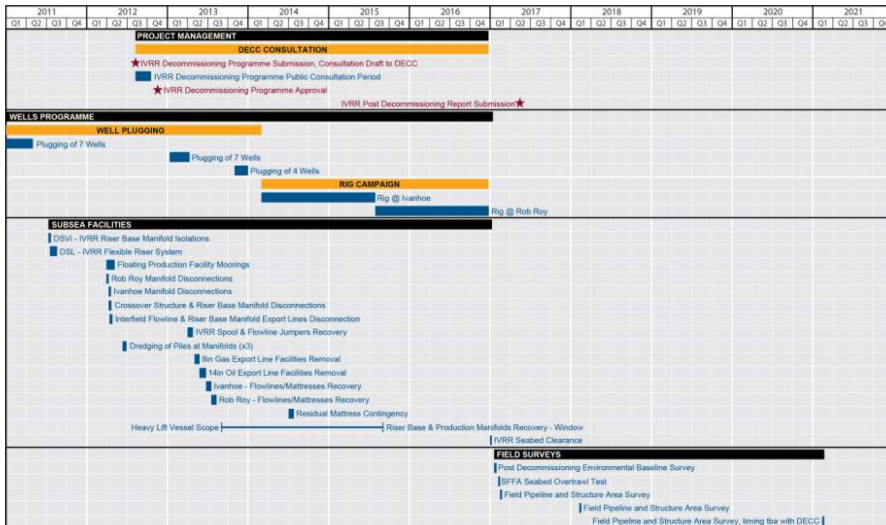
Figure 13.1: Outline Schedule for Phase 3 Full IVRR Decommissioning Project
