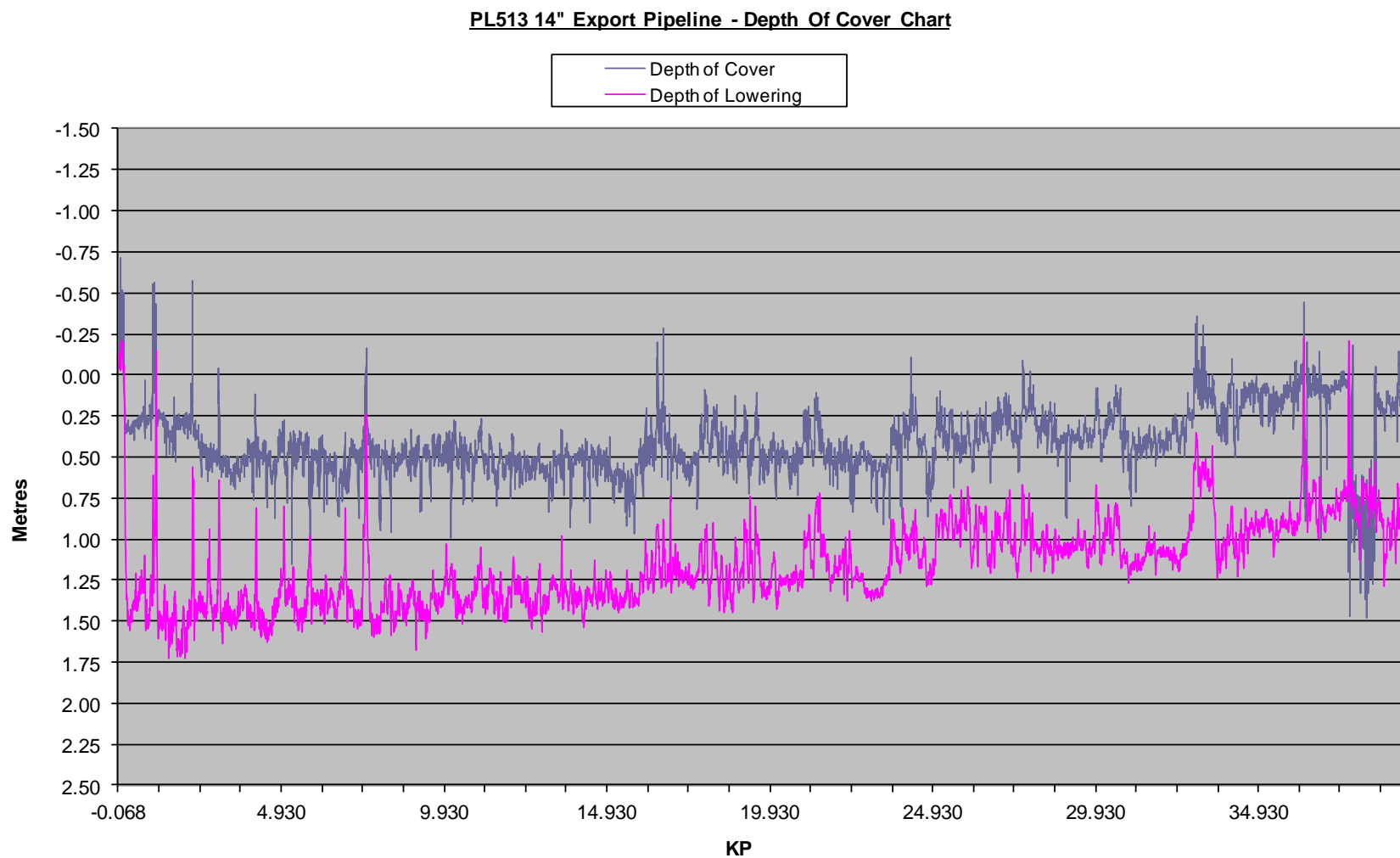
Figure 4.7: PL513 Position within the Seabed and Level of Cover as found during 2012 Survey
