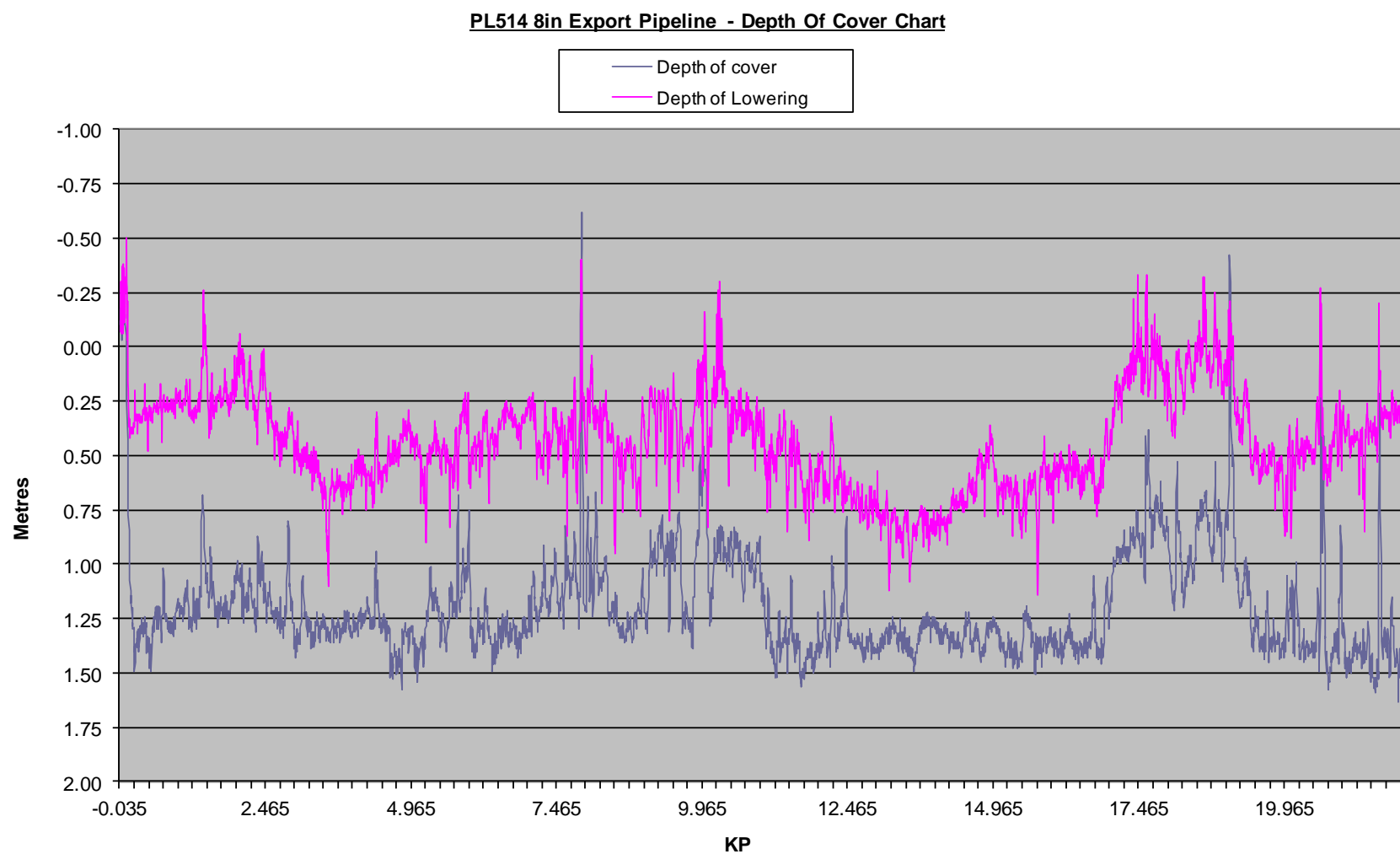
Figure 4.8: PL514 Position within the Seabed and Level of Cover as found during 2012 Survey
