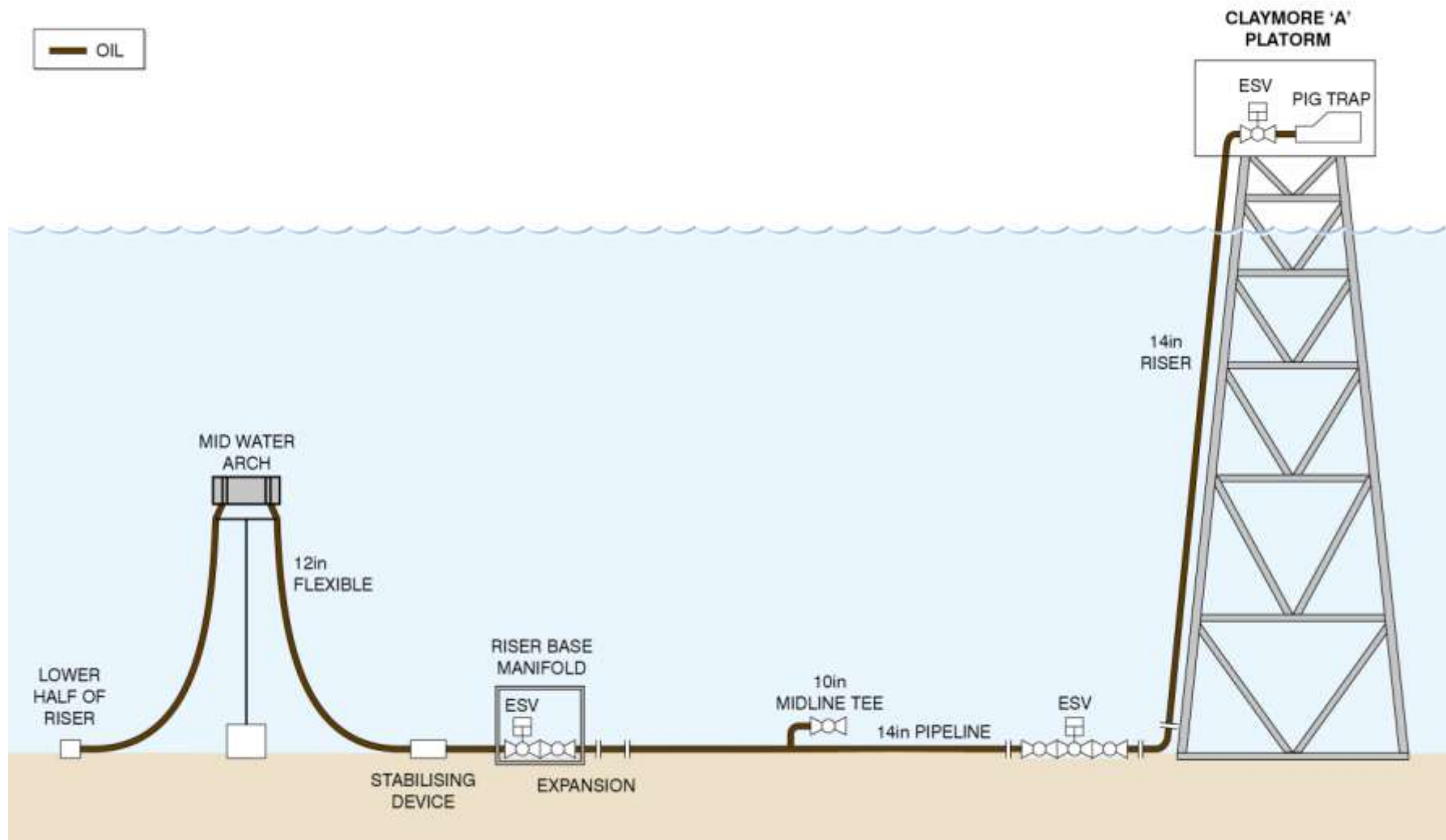
Figure 4.5: Oil Export System During Field Operation (MWA and Flexible Risers have now been removed; schematic does not show areas of burial and is not to scale)
