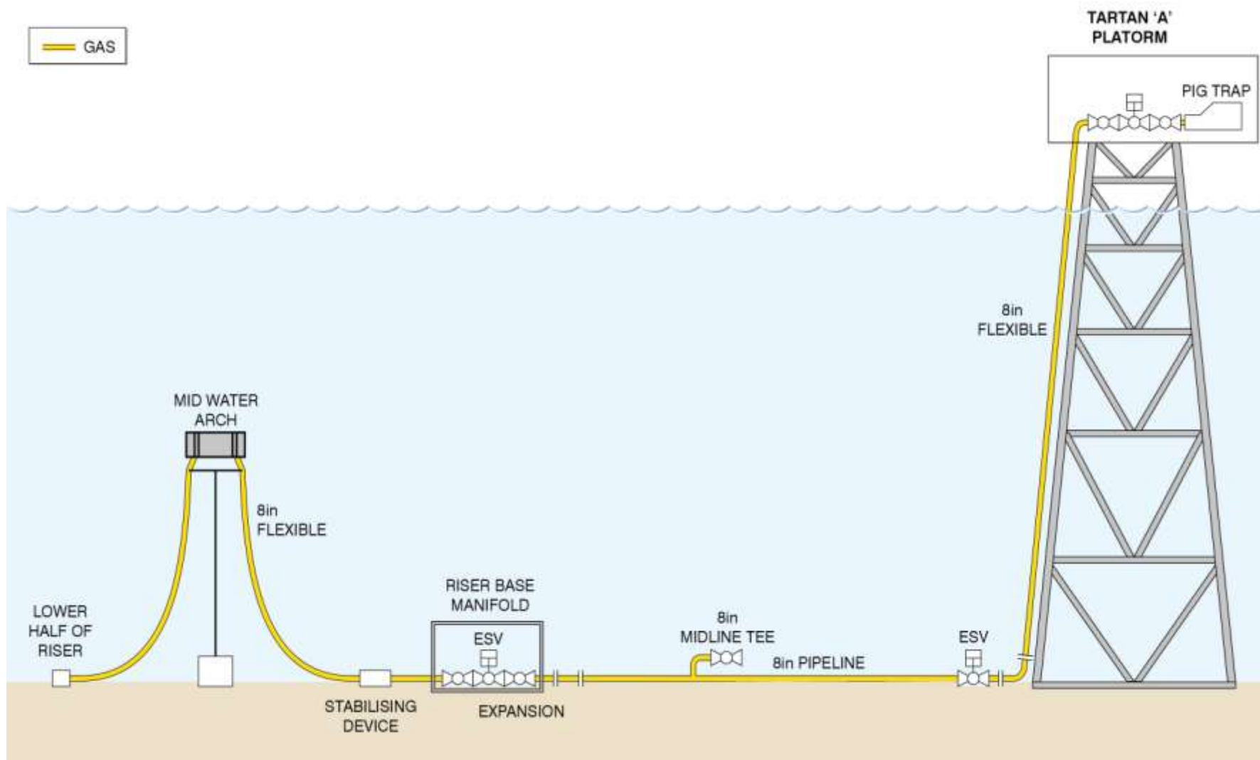
Figure 4.6: Gas Import/Export System During Field Operation (MWA and Flexible Risers have now been removed; schematic does not show areas of burial and is not to scale)
