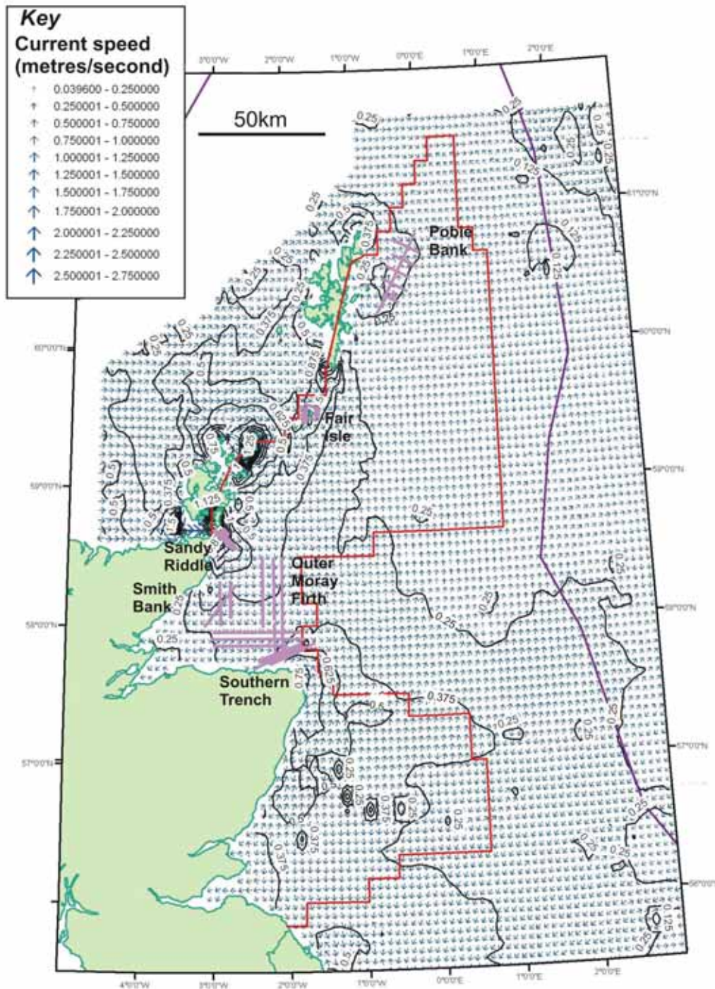
Figure 17. Mean peak spring-tide near-bed current speeds and directions. The data has been generated using the POLCOMS model described by Holt and James (2001) for stormy (October) conditions. Locations of the main DTI 2003 surveys are outlined schematically in purple.
