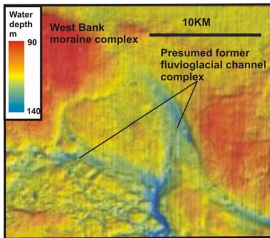
Figure 8. West Bank: Interpretations of possible former terrestrial moraine and fluvio-glacial channel complex. Image generated from seabed picks of multichannel data from 3D commercial surveys. See Figures 7, 8 for location. The topographic boundary separating the West Bank moraine complex from the former fluvio-glacial channel complex possibly marks the site of a former terrestrial ice margin.
