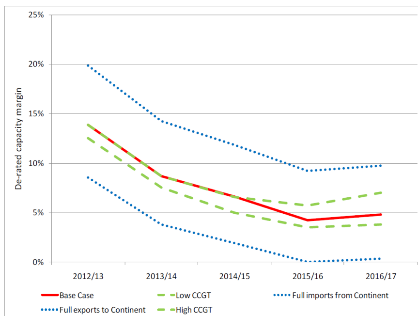
Figure 4: Ofgem estimates of de-rated capacity margins
