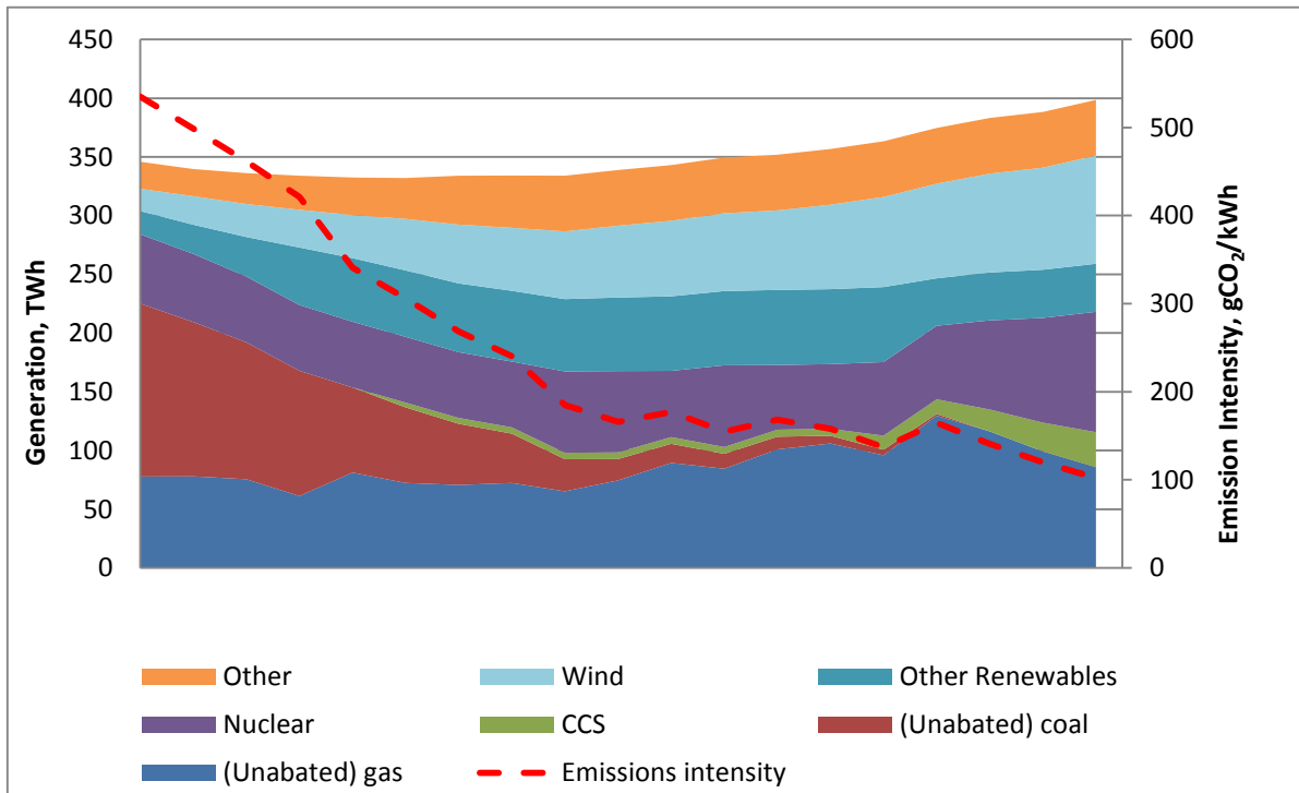
Figure 7: Type and carbon intensity of electricity generation in the basecase
