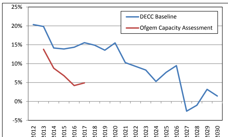
Figure 5: Ofgem and DECC estimates of de-rated capacity margins
