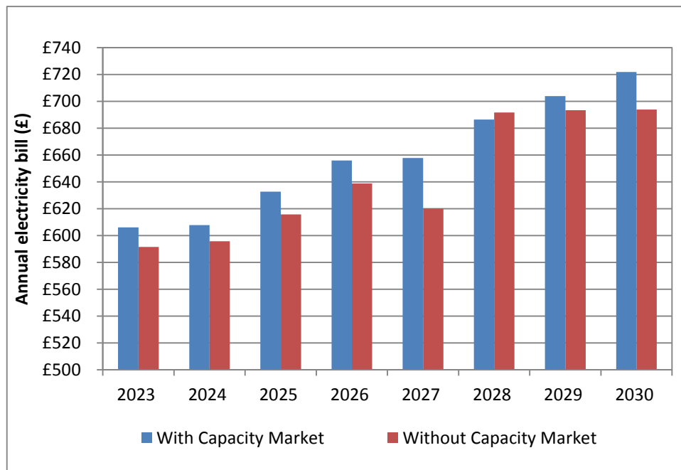
Figure 11: Change in Domestic Electricity Bills in the Base Case
