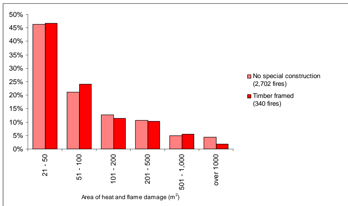
Chart 2: Distribution of heat and flame damage over 20m 2 in fires in non-residential buildings, England, April 2009-March 2012
