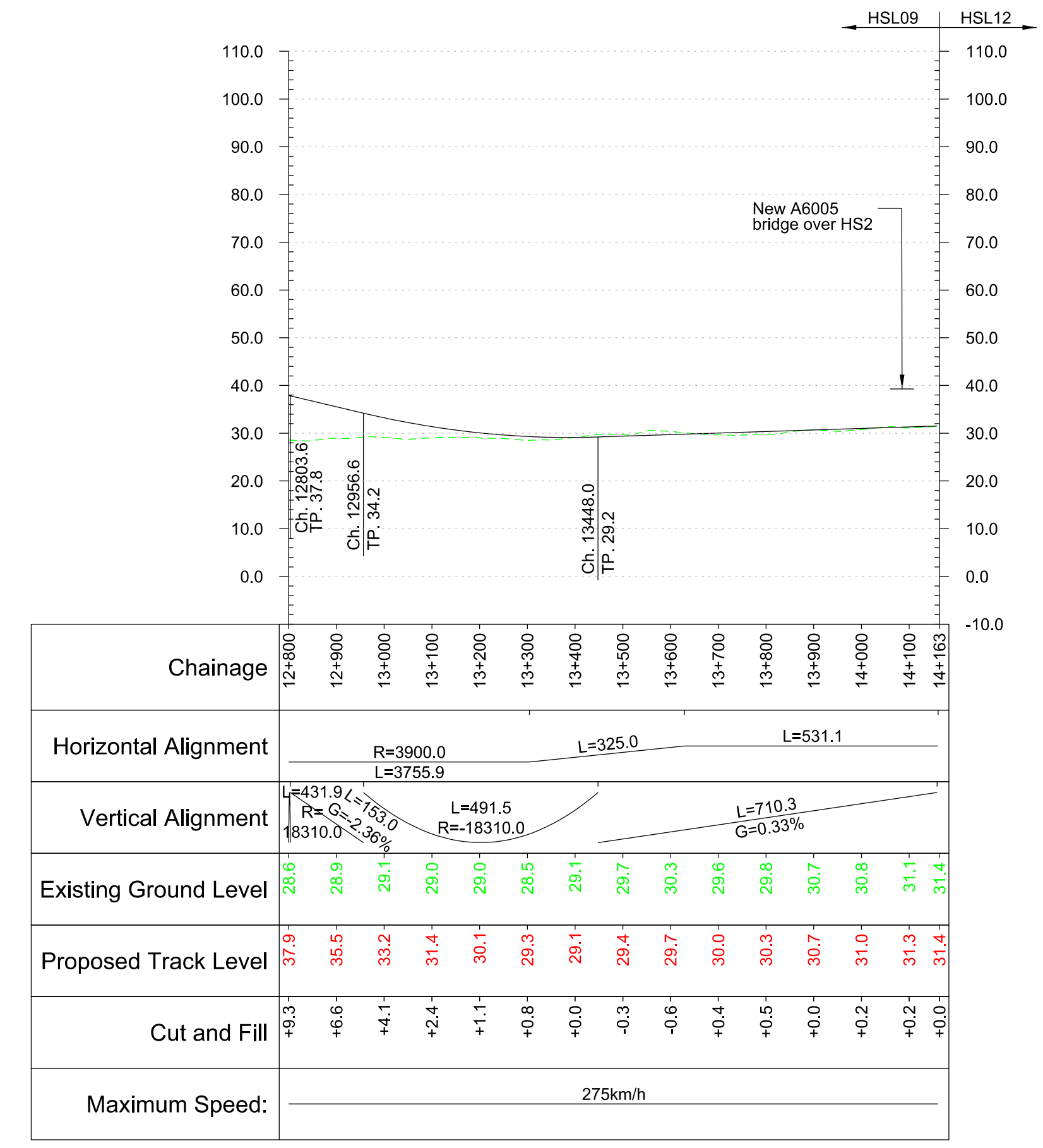
Profile Scale H 1:10000 V 1:1000 @ A1
