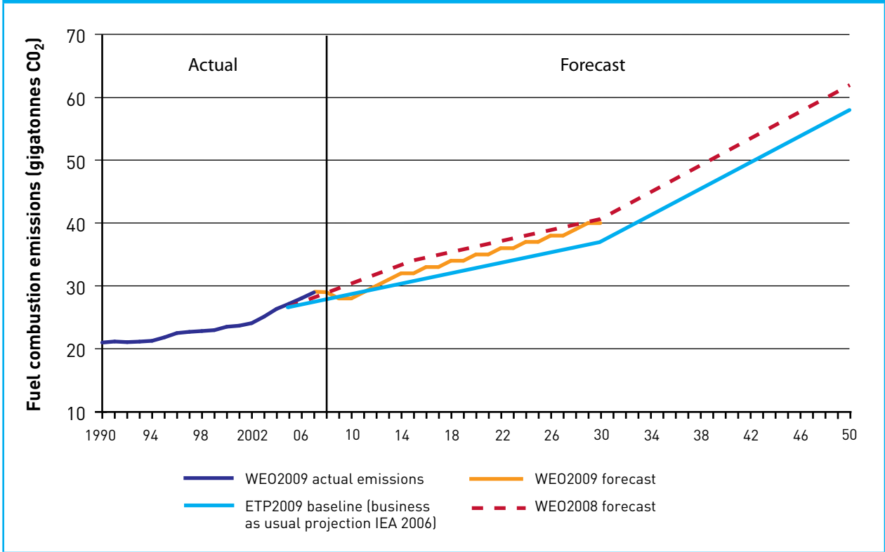
Figure A.1: Global CO 2 emissions from fuel combustion, actual and forecast
