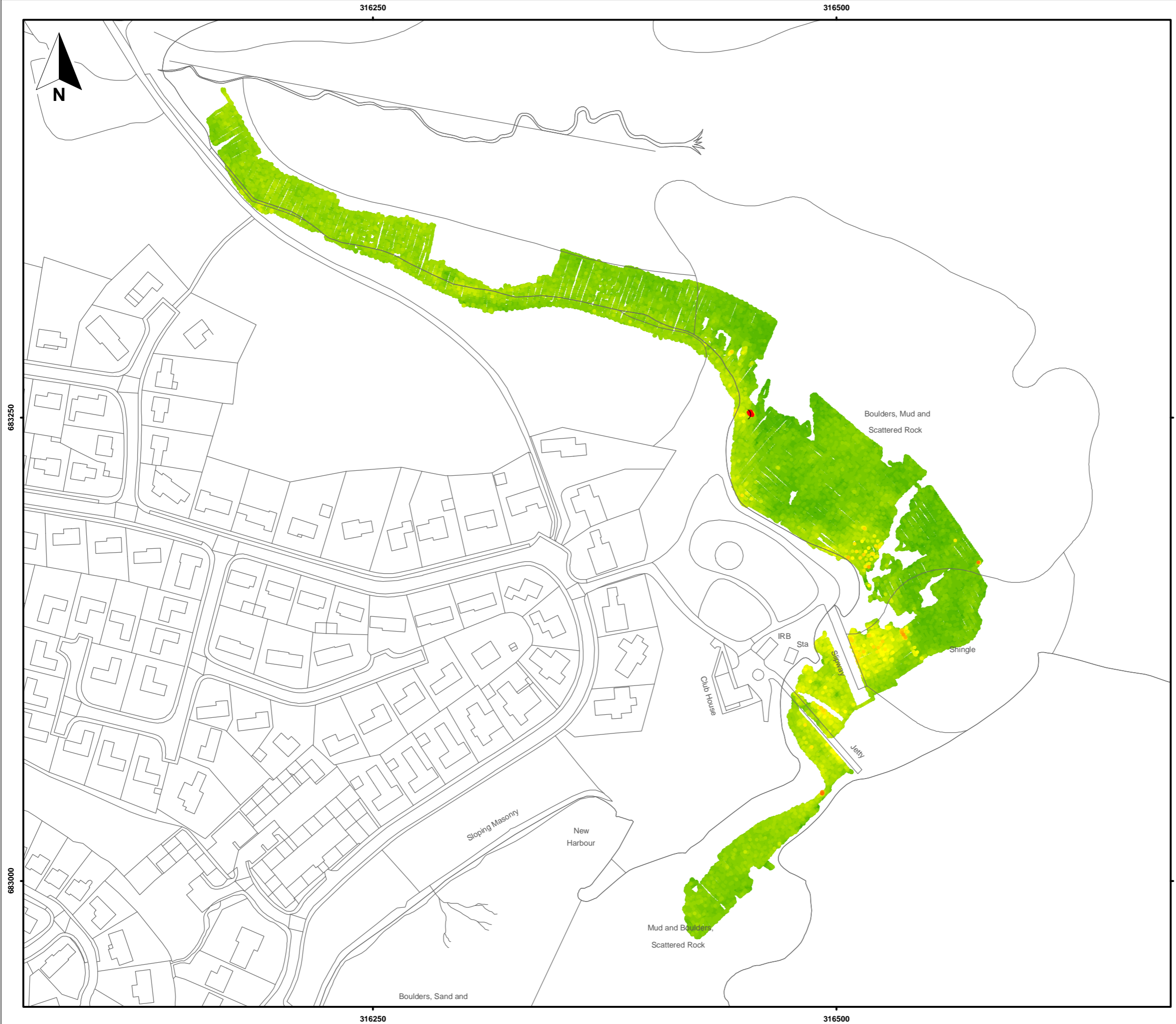
Figure 13 Monitoring Survey 4 (3-5/03/2010): Measured Activity Levels
