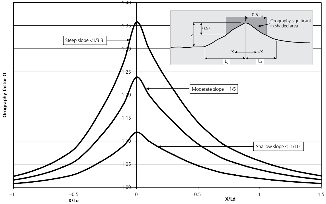
Figure 3a Orography Factor O for hills and ridges (interpolation between curves may be used)
