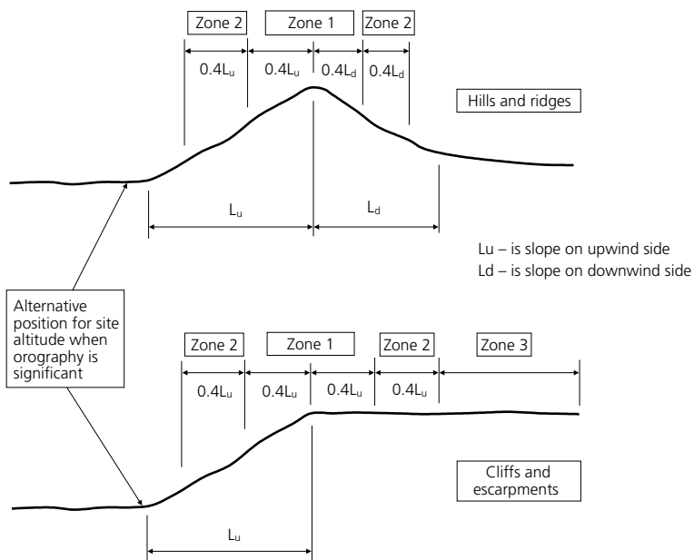
Figure 2 Orographic zones for Factor O
