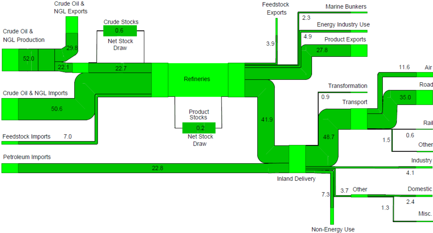
Chart H.2: Petroleum flow chart 2011 (million tonnes)
