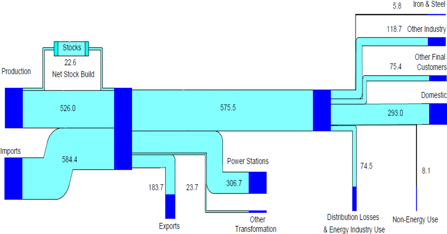
Chart H.3: Natural gas flow chart 2011 (TWh)
