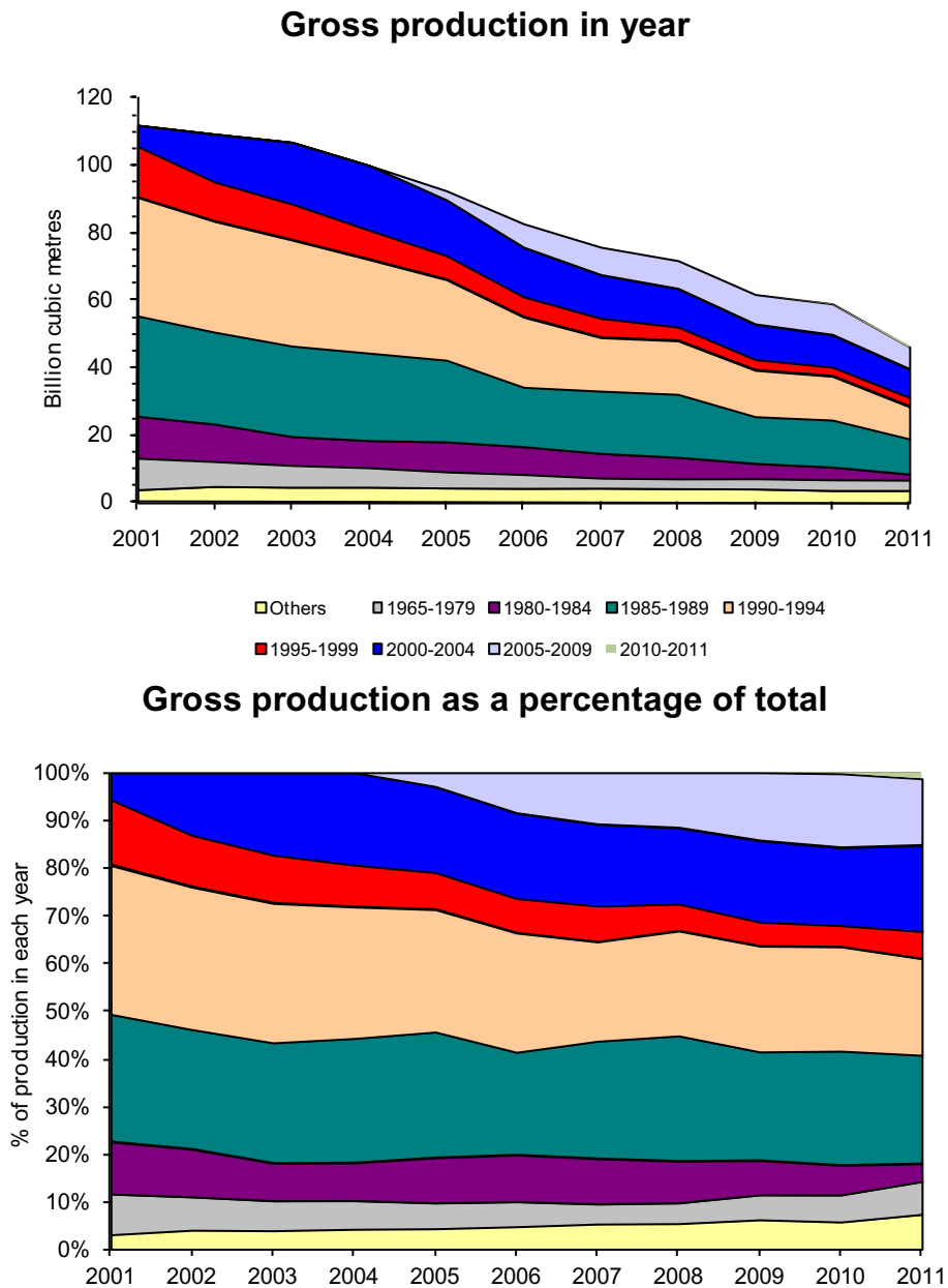
Chart F.5: Age profile of gross UK gas production
