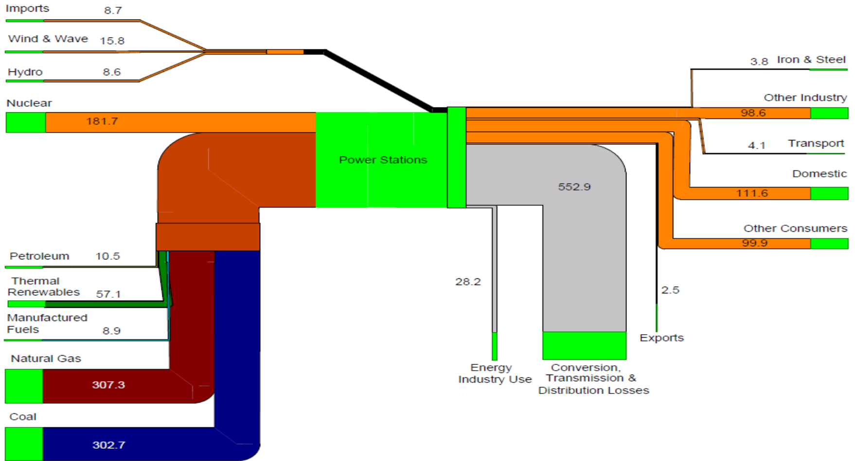
Chart H.4: Electricity flow chart 2011 (TWh)
