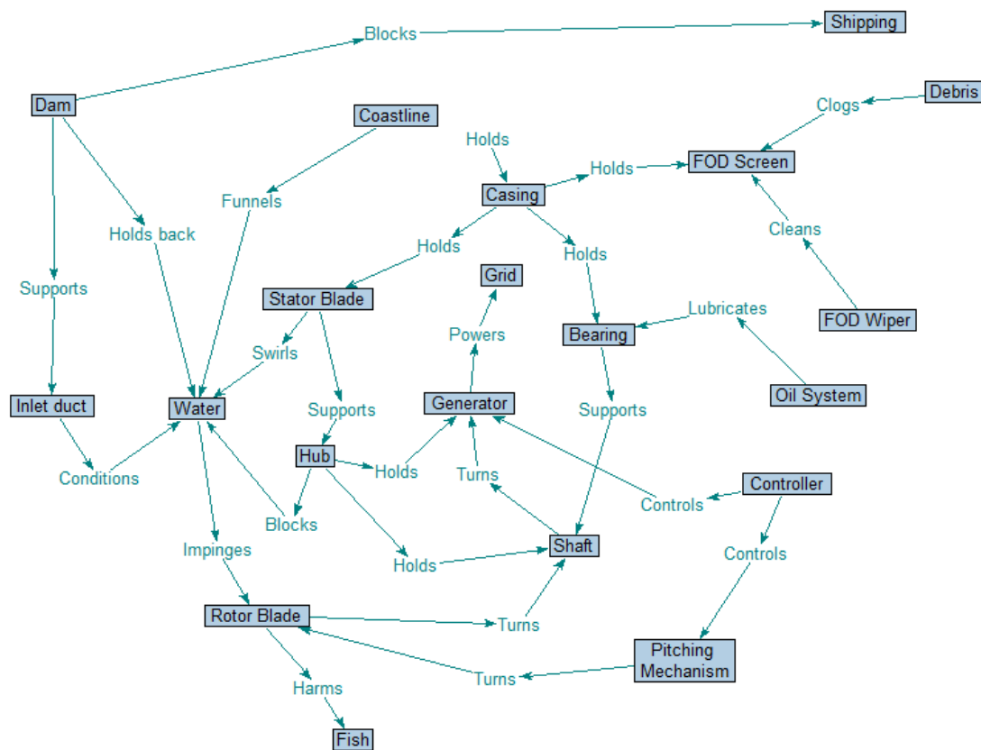
Figure 2 Functional analysis diagram showing the decomposition of a turbine system into its key components and illustrating their functional interactions.
