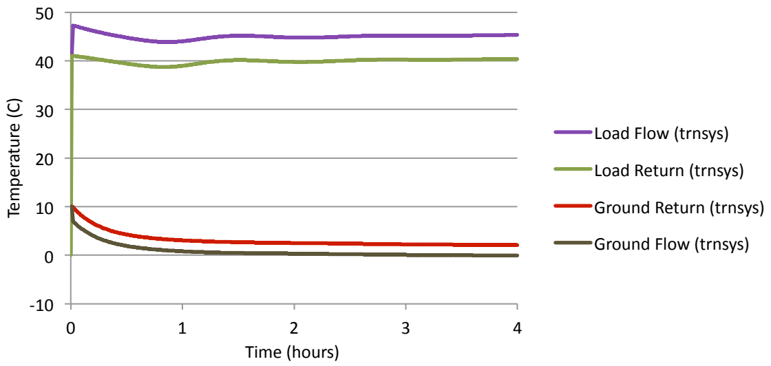
Figure 5: Ground and load side temperatures from Trnsys for a "continuous run"
