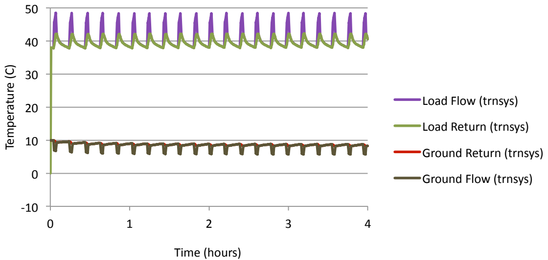
Figure 6: Ground and load side temperatures from Trnsys for a "short cycle" run
