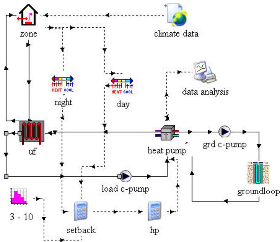
Figure 23: Trnsys model - underfloor heating with night setback
