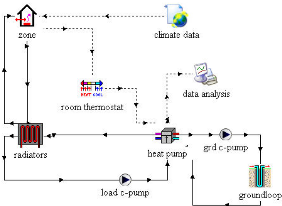
Figure 4: Schematic of the Trnsys model used to simulate the GSHP system.
