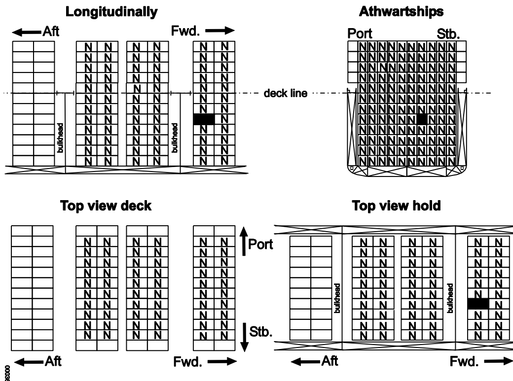
3 – Situation open versus open – UNDER DECK Note: All bulkheads and decks shall be resistant to fire and liquids.
