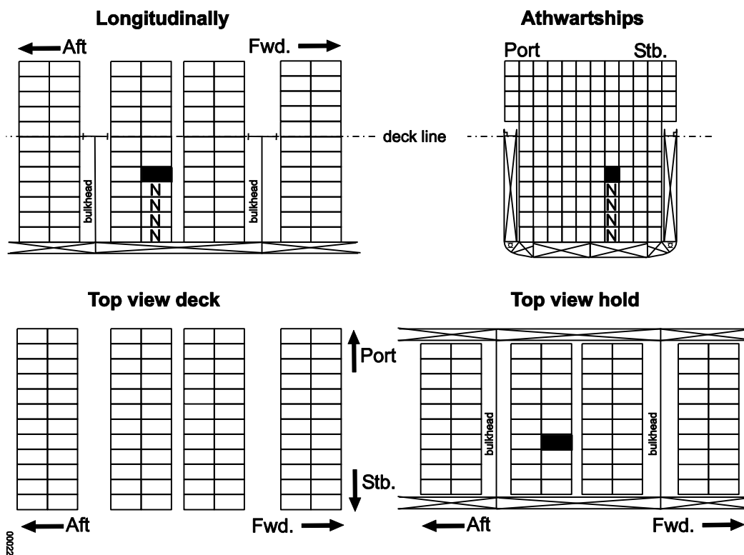
1 – Situation closed versus open – UNDER DECK Note: All bulkheads and decks shall be resistant to fire and liquids.
