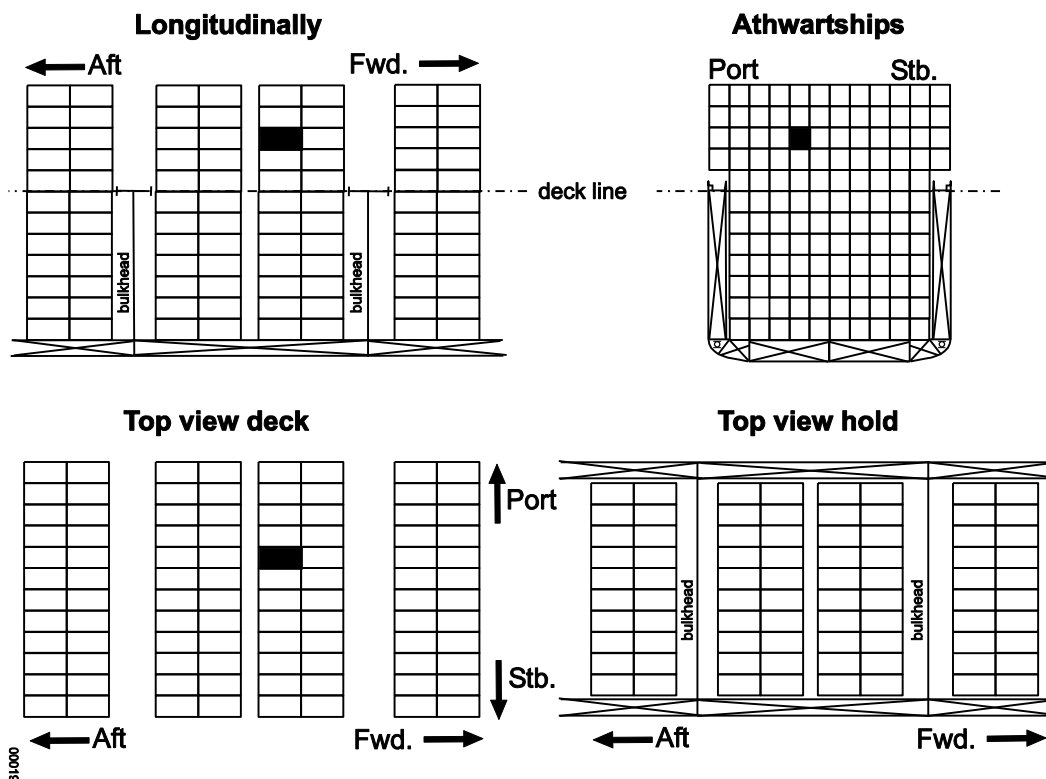
1 – Situation closed versus closed – ON DECK Note: All bulkheads and decks shall be resistant to fire and liquids.
