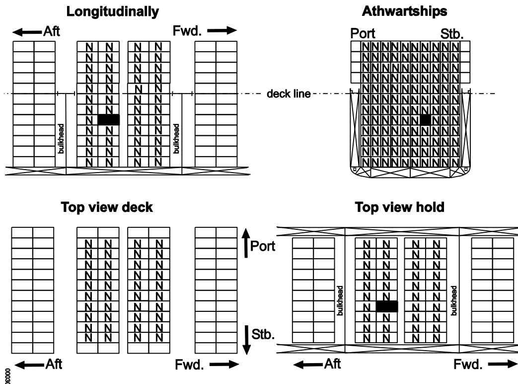
2 – Situation open versus open – UNDER DECK Note: All bulkheads and decks shall be resistant to fire and liquids.
