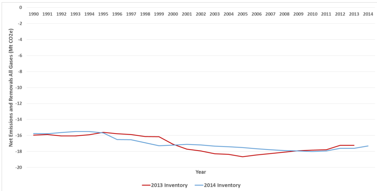
Figure 6.5 4A Forest Land changes in net emissions between 2013 and 2014 inventories
