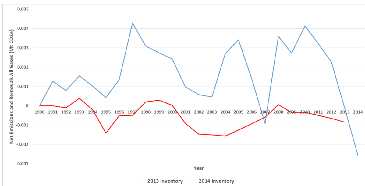
Figure 6.13 LULUCF sector change in net emissions between the 1990-2013 and 1990-2014 inventories for Jersey
