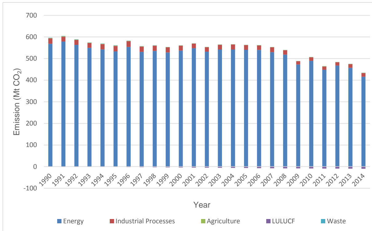
Figure 2.2 UK CO 2 Emissions Trend by Sector for 1990 to 2014
