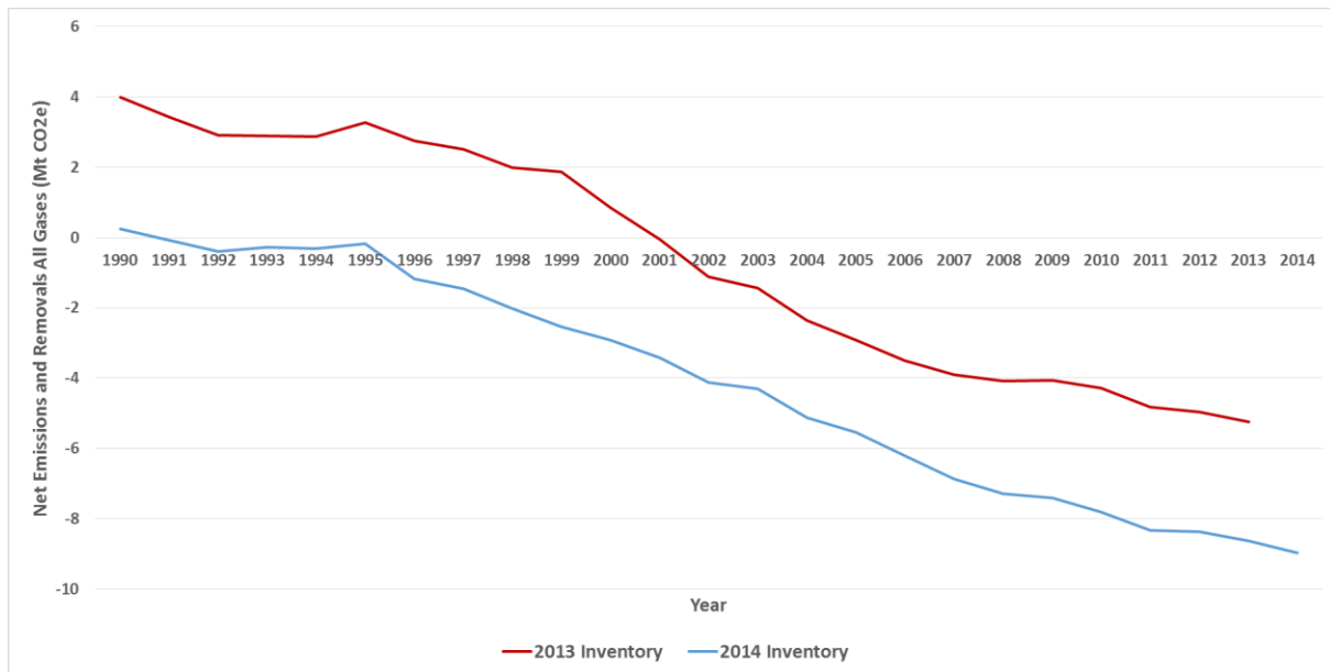
Figure 6.1 LULUCF change in net emissions for all gases between the 2013 and 2014 inventories
