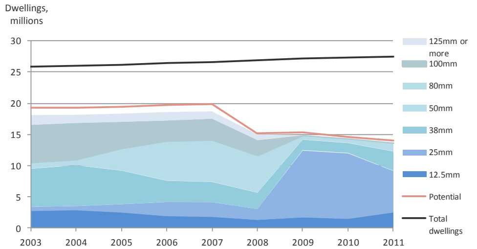
Graph 6q: Hot water tank insulation – post GfK survey
