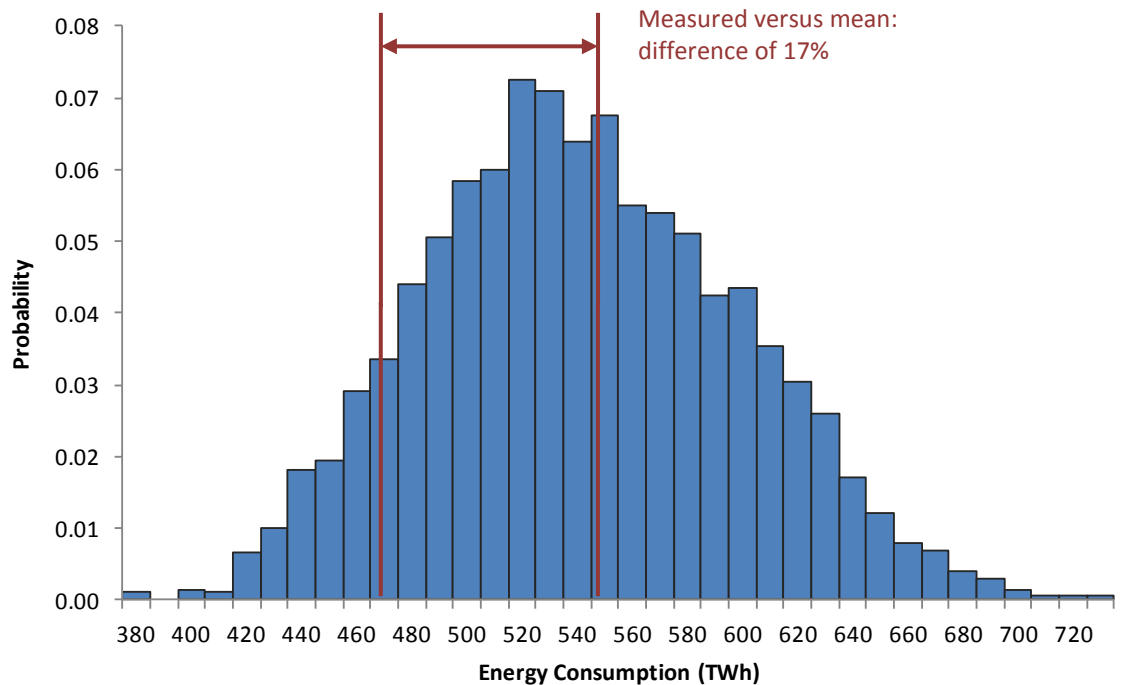
Monte Carlo distributions of total English domestic energy consumption in 2010 using the CHM. The 'measured' value from DUKES is 463 TWh and the difference between this and our mean is 17%.
