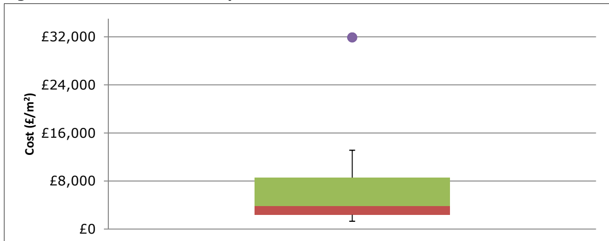
Figure A.18: Box and Whisker plot for MVHR
