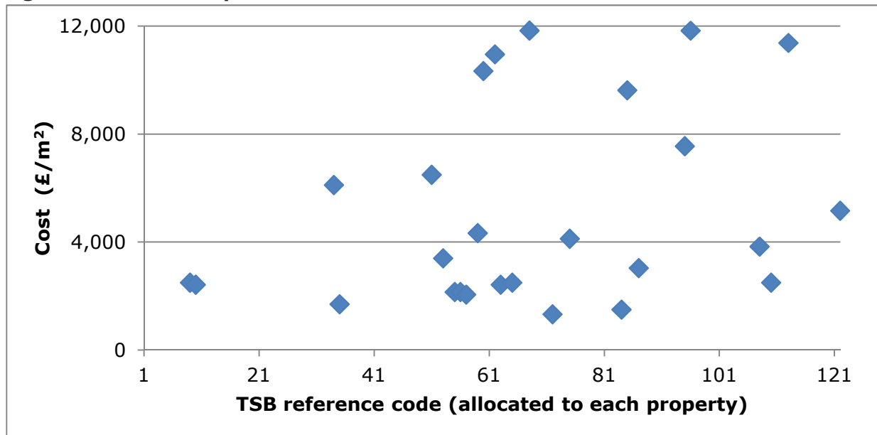
Figure A.17: Scatter plot for MVHR
