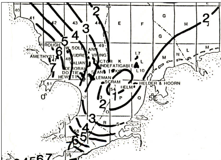
Figure C3.2 Propagation of tides
