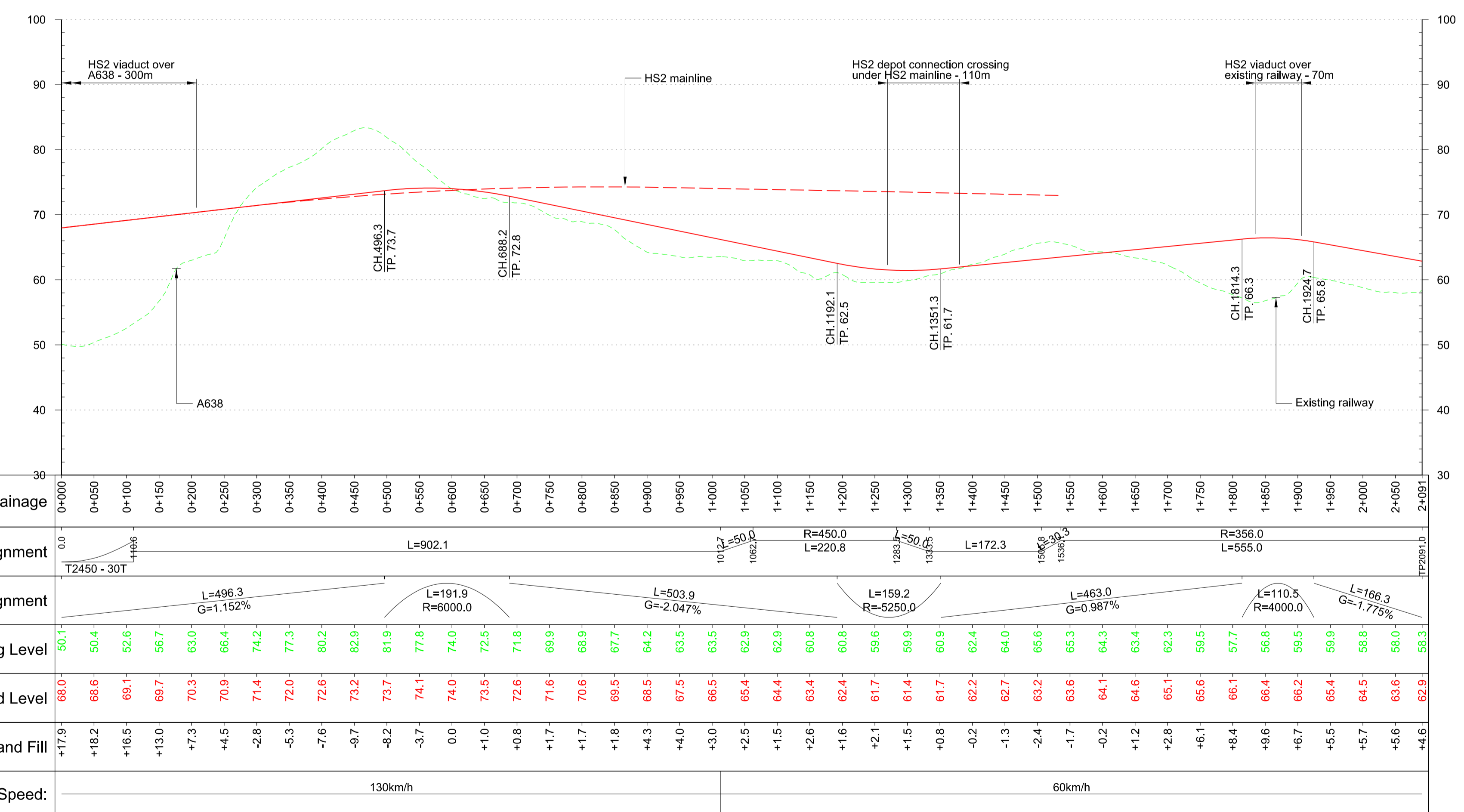
Profile Scale H:1:5,000 V:1:500 @ A1
