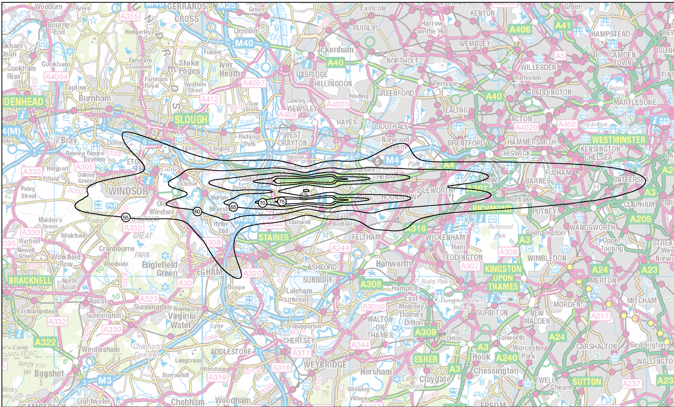
H40-2R: Heathrow 2040 do-minimum Annual average Lden
