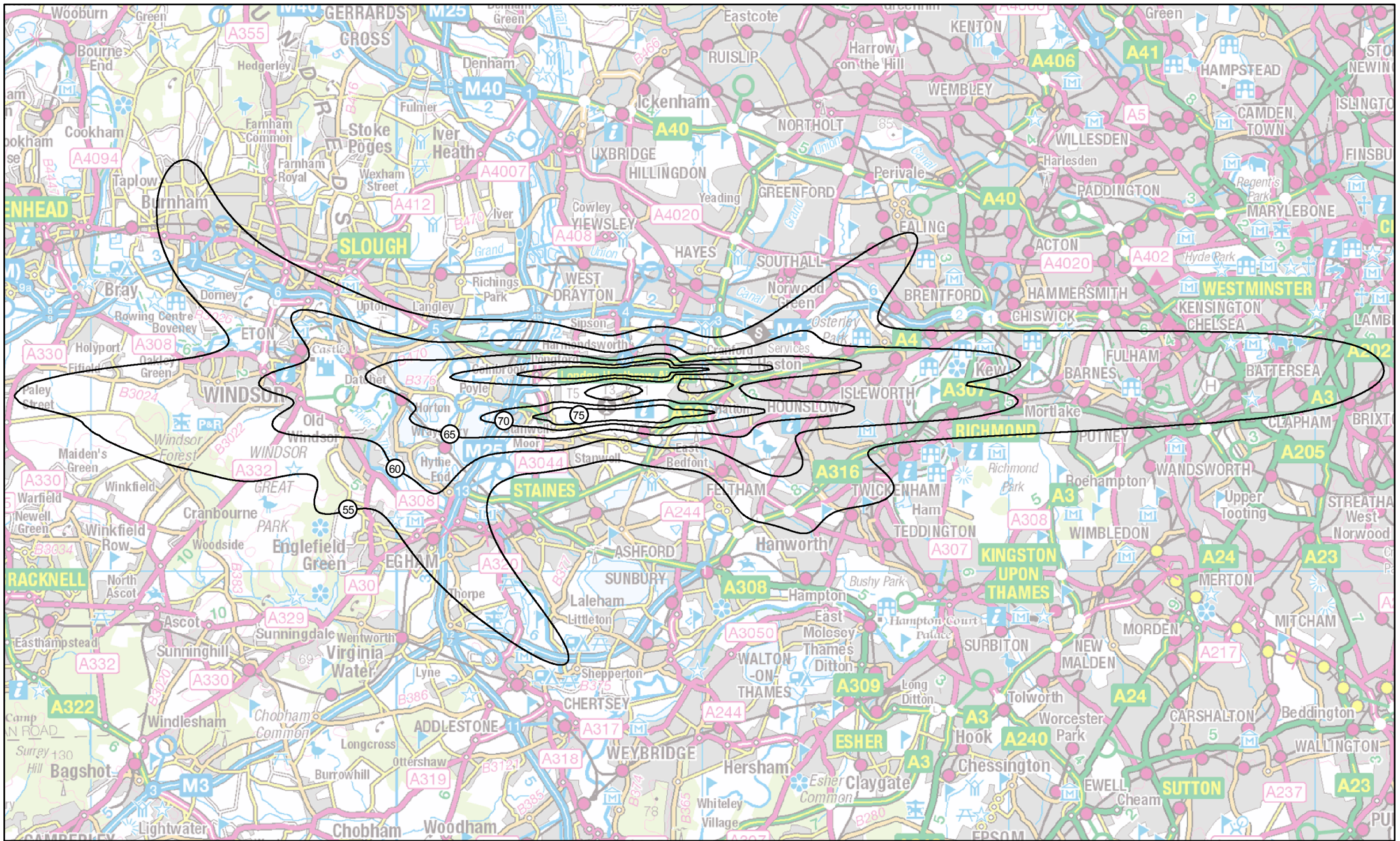
H11-2R: Heathrow 2011 current, actual modal split Annual average Lden
