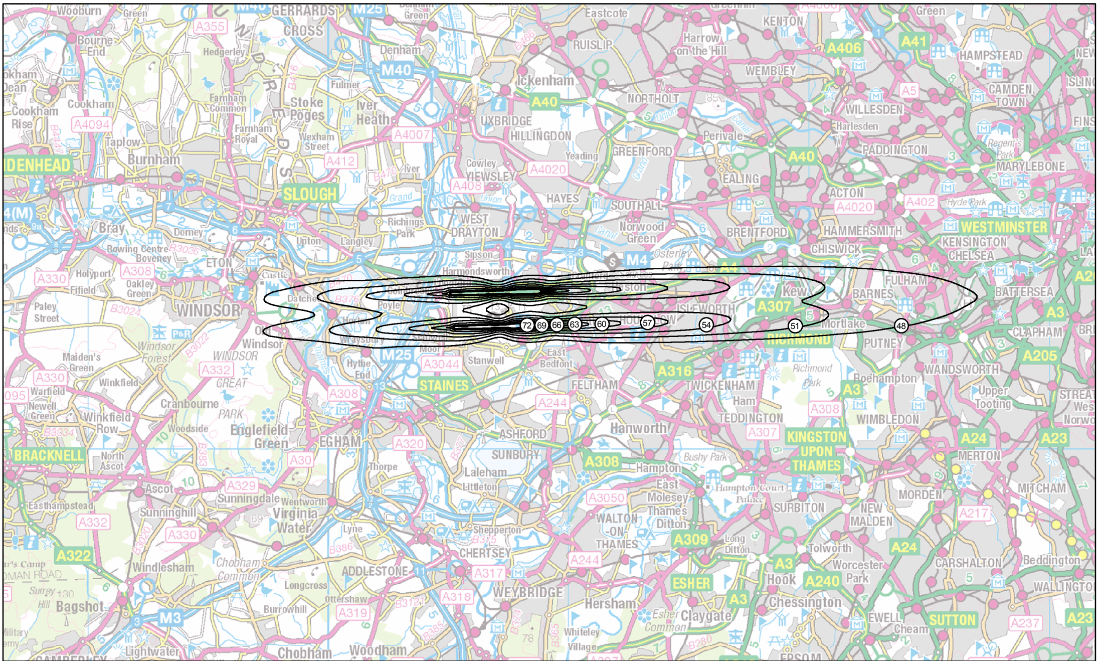
H40-2R: Heathrow 2040 do-minimum Summer average 8-hour night-time LAeq,8h
