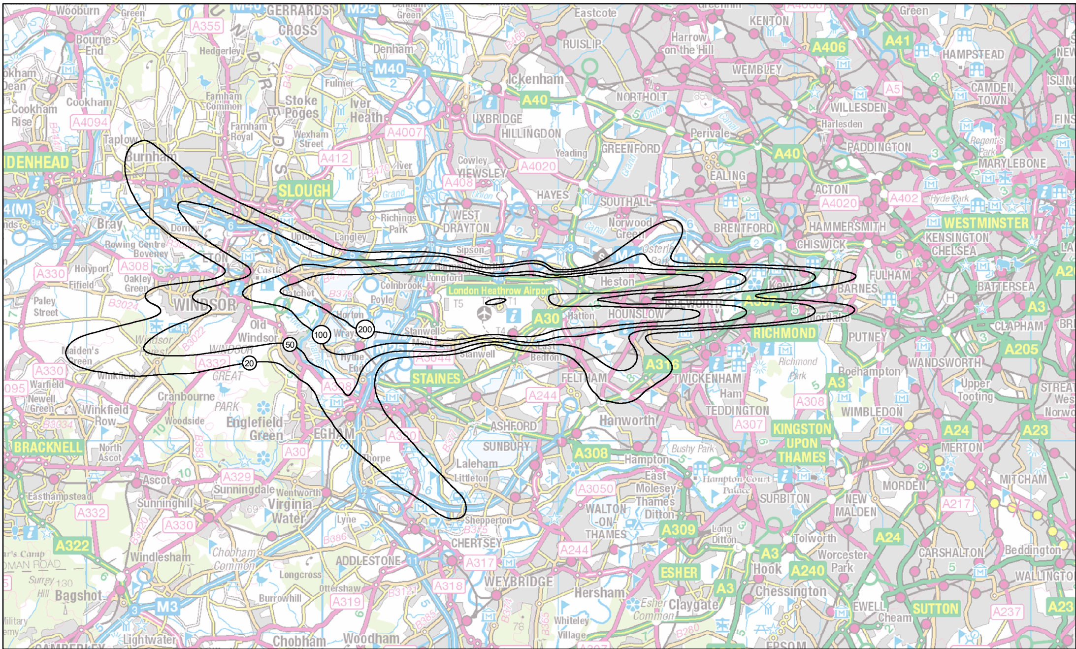
H13-2R: Heathrow 2013 current, standard modal split Summer average daytime N70
