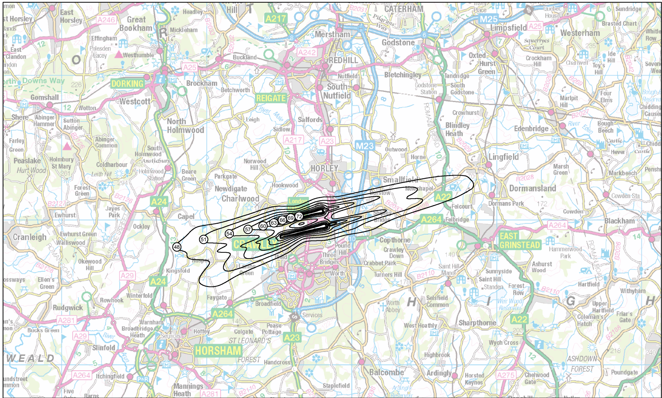
G50-2R-X-QC: Gatwick 2030 do-something, GAL - No core night operations Summer average 8-hour night-time LAeq,8h
