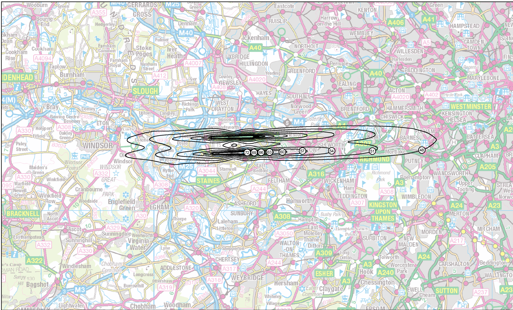
H30-2R: Heathrow 2030 do-minimum Summer average 8-hour night-time LAeq,8h
