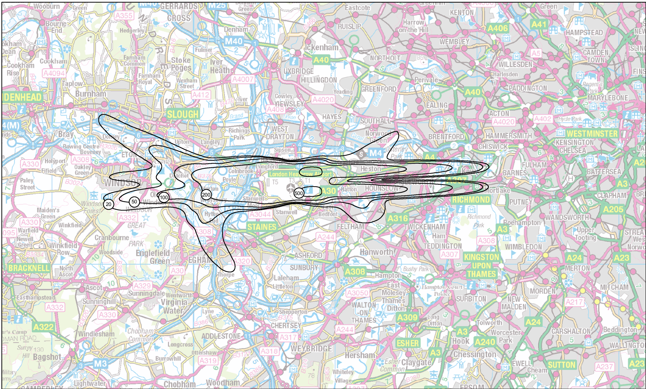
H30-2R: Heathrow 2030 do-minimum Summer average daytime N70
