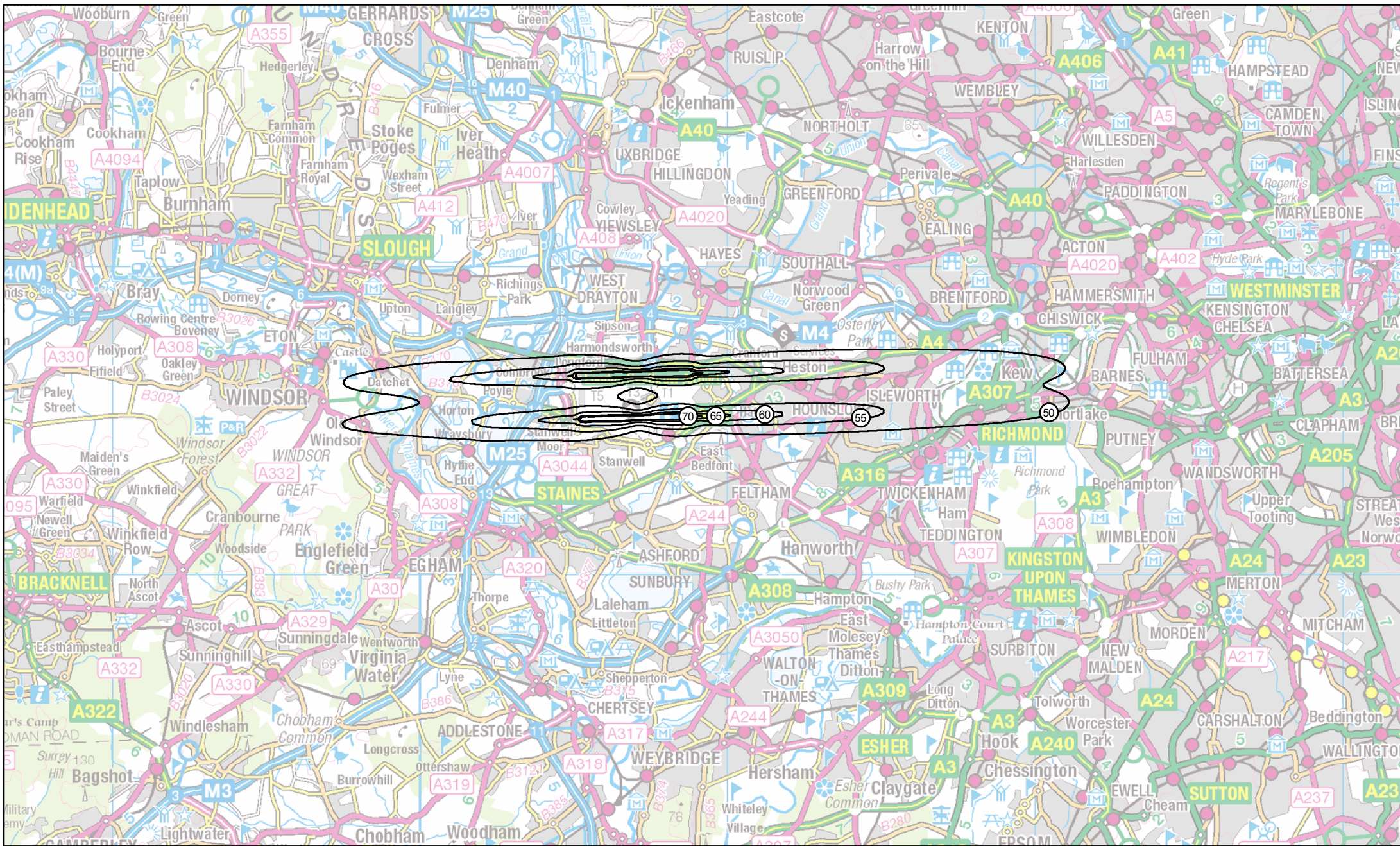
H30-2R: Heathrow 2030 do-minimum Annual average Night
