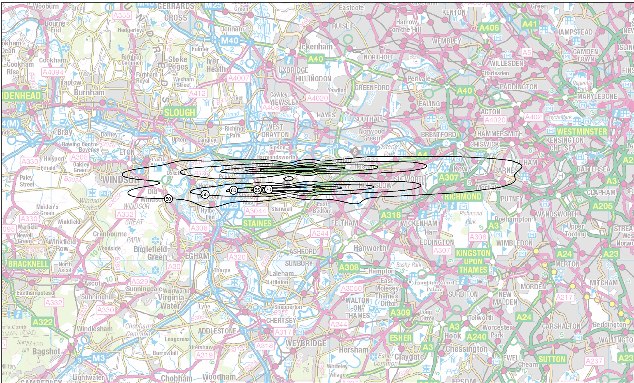
H11-2R: Heathrow 2011 current, actual modal split Annual average Nlight
