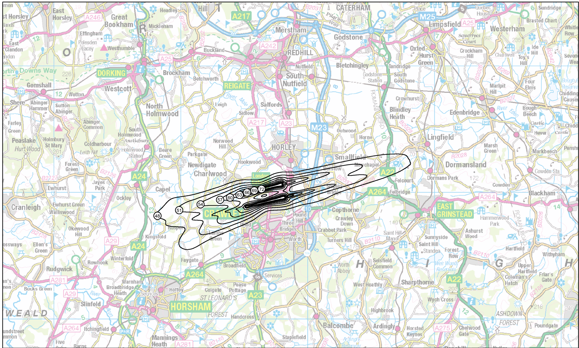
G40-2R-X-QC: Gatwick 2030 do-something, GAL - No core night operations Summer average 8-hour night-time LAeq,8h
