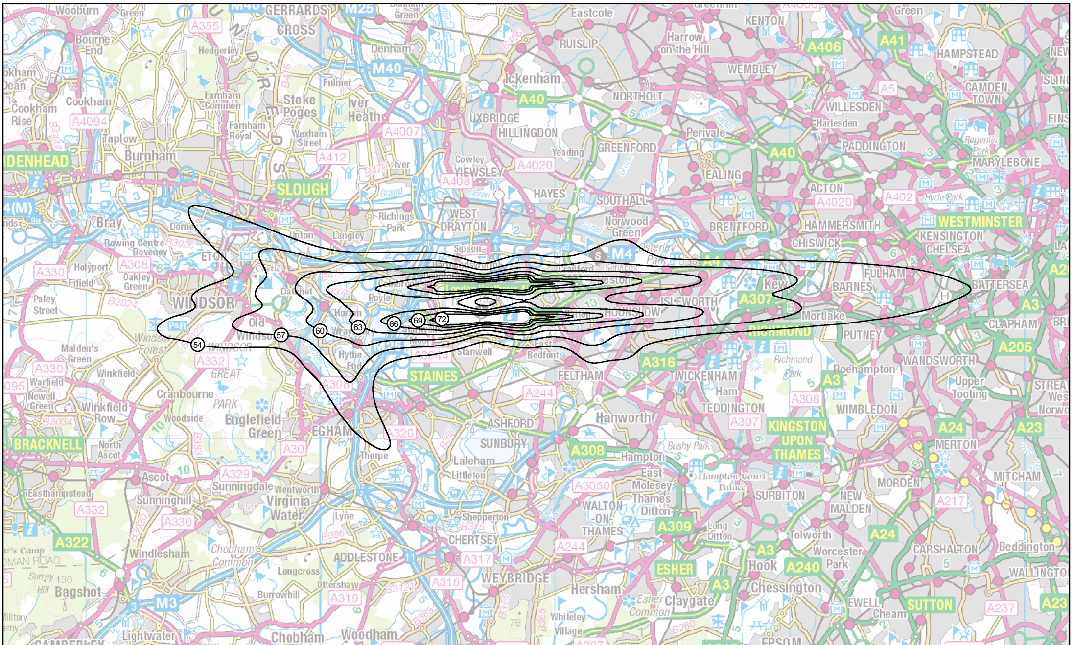
H40-2R: Heathrow 2040 do-minimum Summer average 16-hour daytime LAeq,16h
