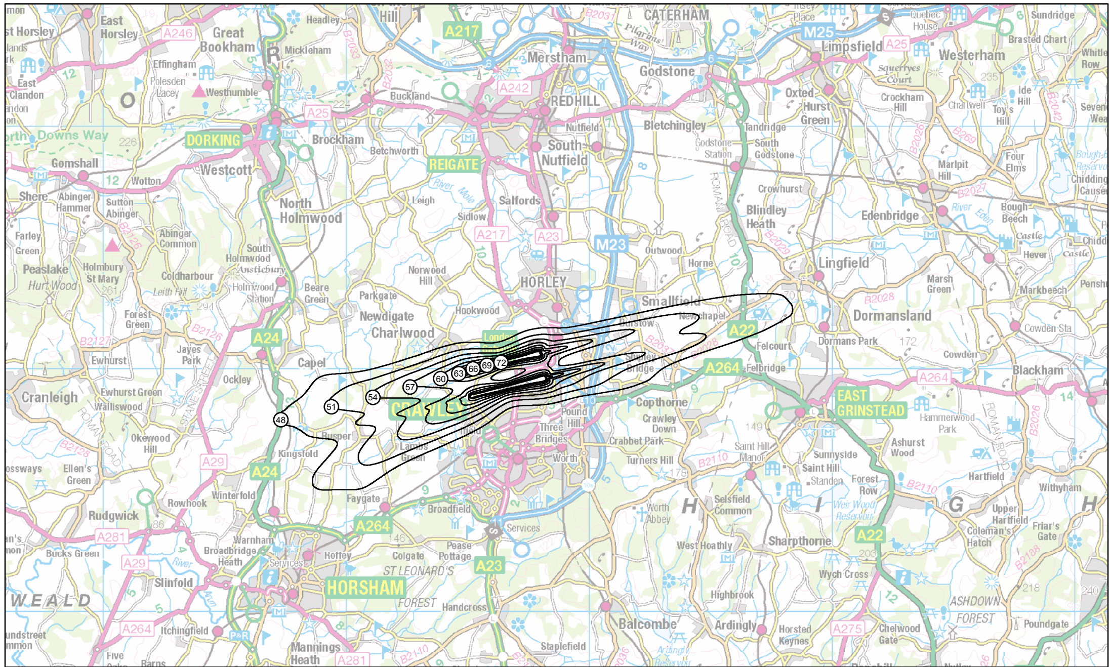
G30-2R-X-QC: Gatwick 2030 do-something, GAL - No core night operations Summer average 8-hour night-time LAeq,8h
