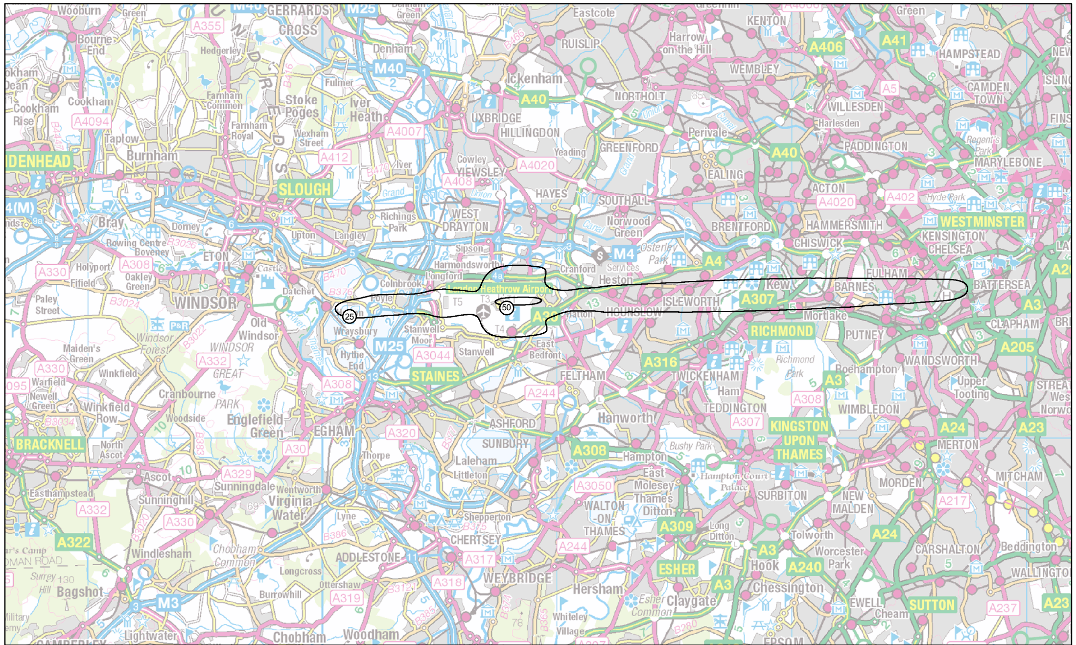
H30-2R: Heathrow 2030 do-minimum Summer average night-time N60
