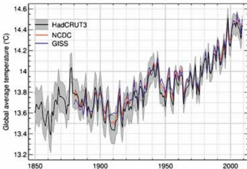
Figure three – Global Average Temperature Record (1850 – Present)
