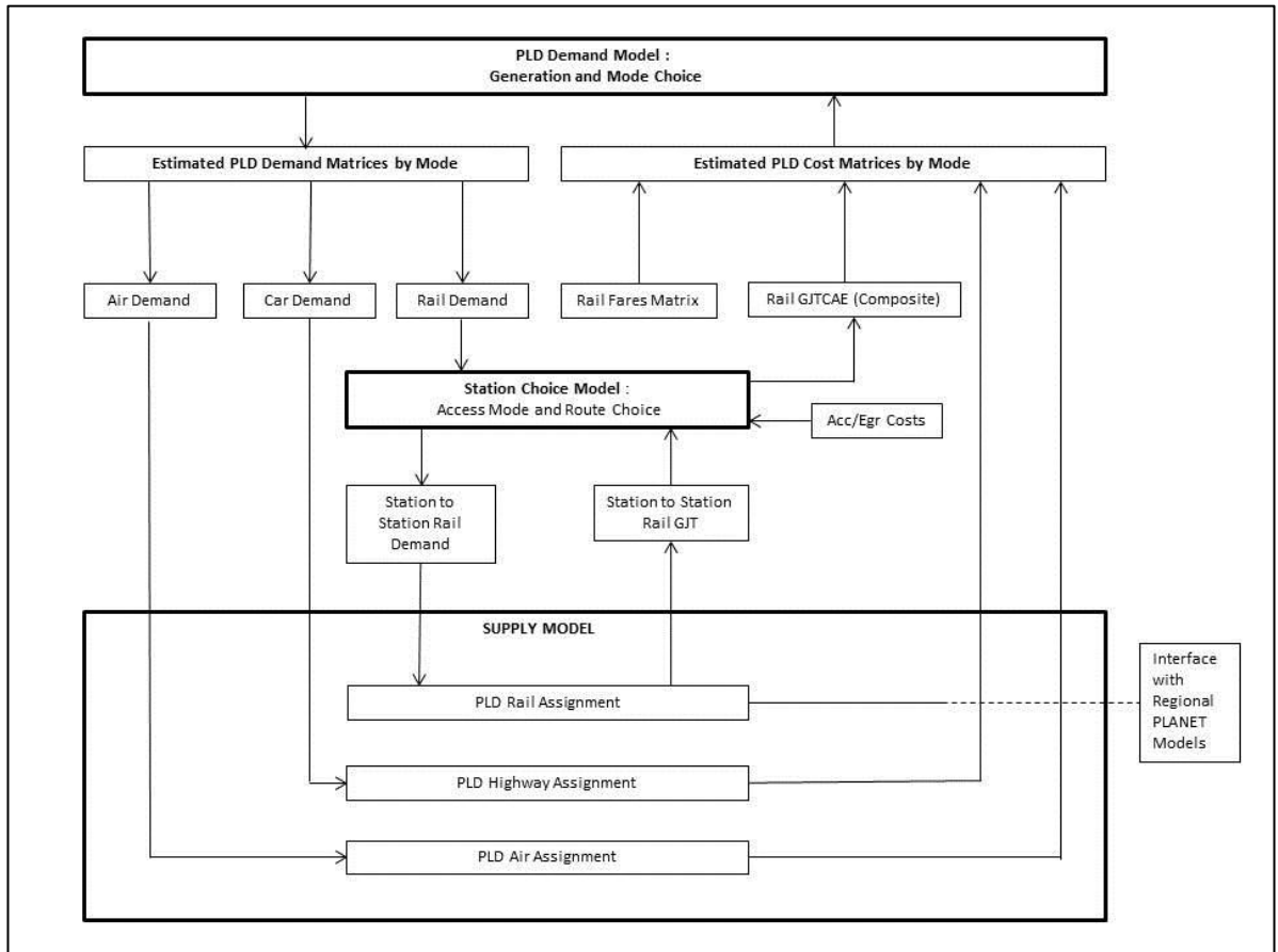
Figure 2-3: PLD Model
