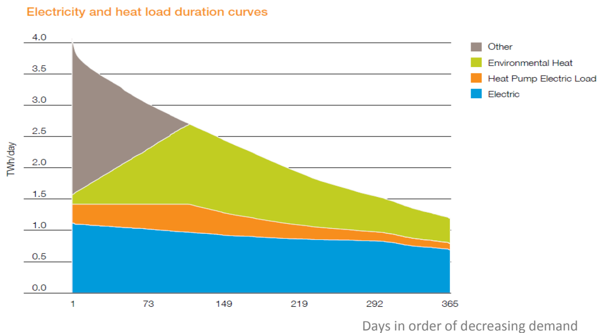
Source: Figure 9, National Grid, Future Energy Scenarios 2012 [21].
