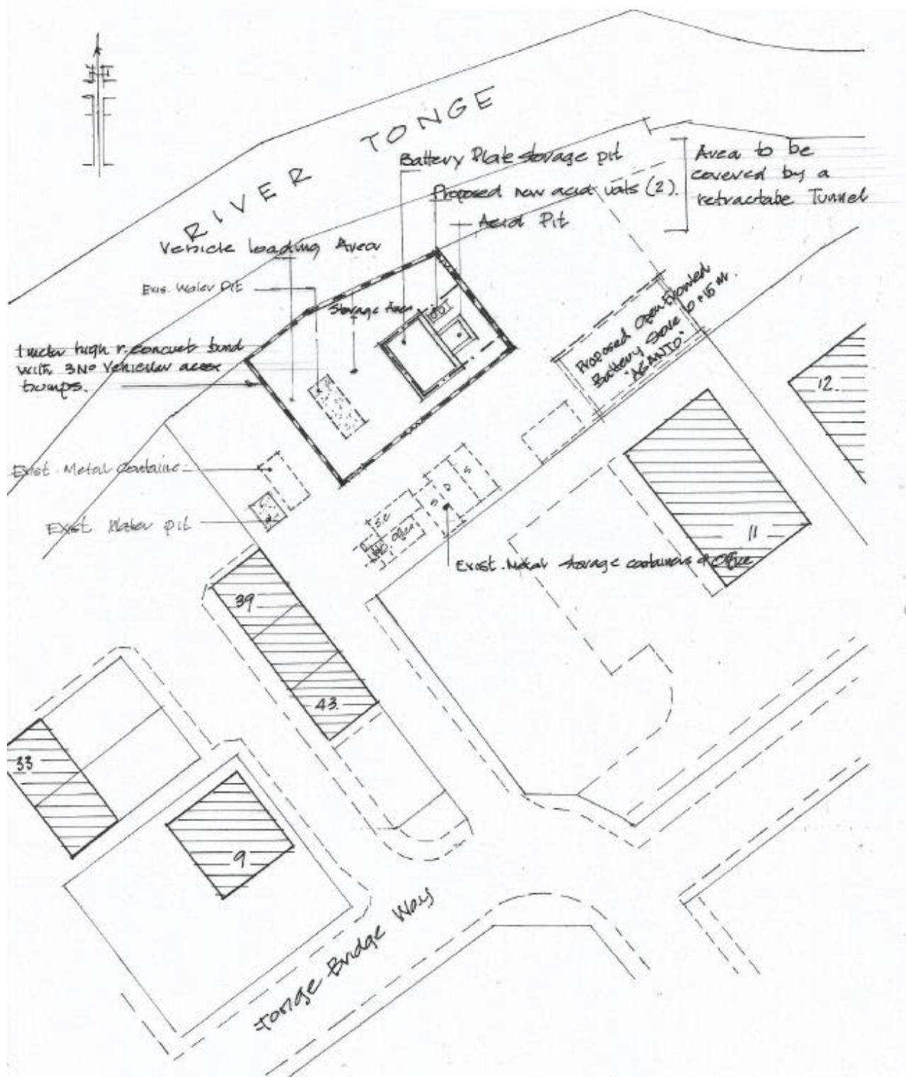
Plot 10 Tonge Bridge Way Bottom (G.M.P. Bawa) Plan showing existing features & new proposals. Scale 1/500
