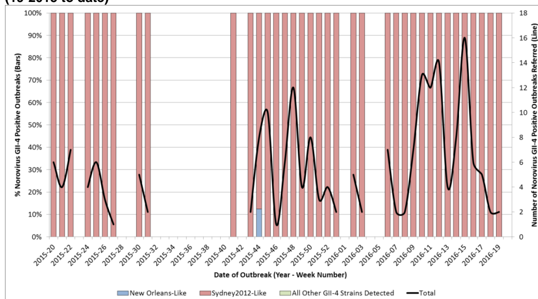
Figure 7: GII-4 norovirus strains detected (by week) among norovirus confirmed outbreaks (all settings) (19-2015 to date)
