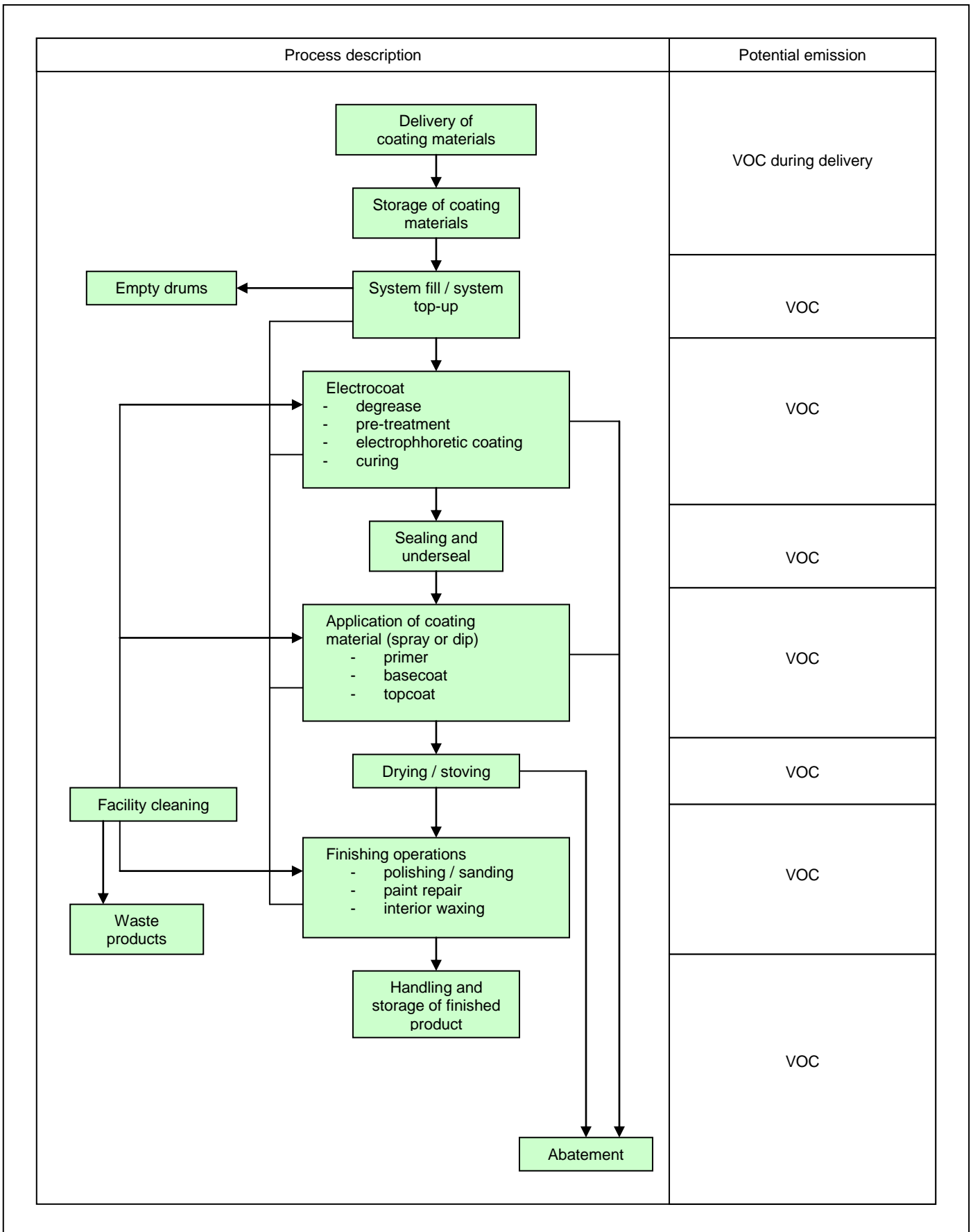
Figure 3.1 - Potential VOC releases from typical paint application in vehicle manufacturing
