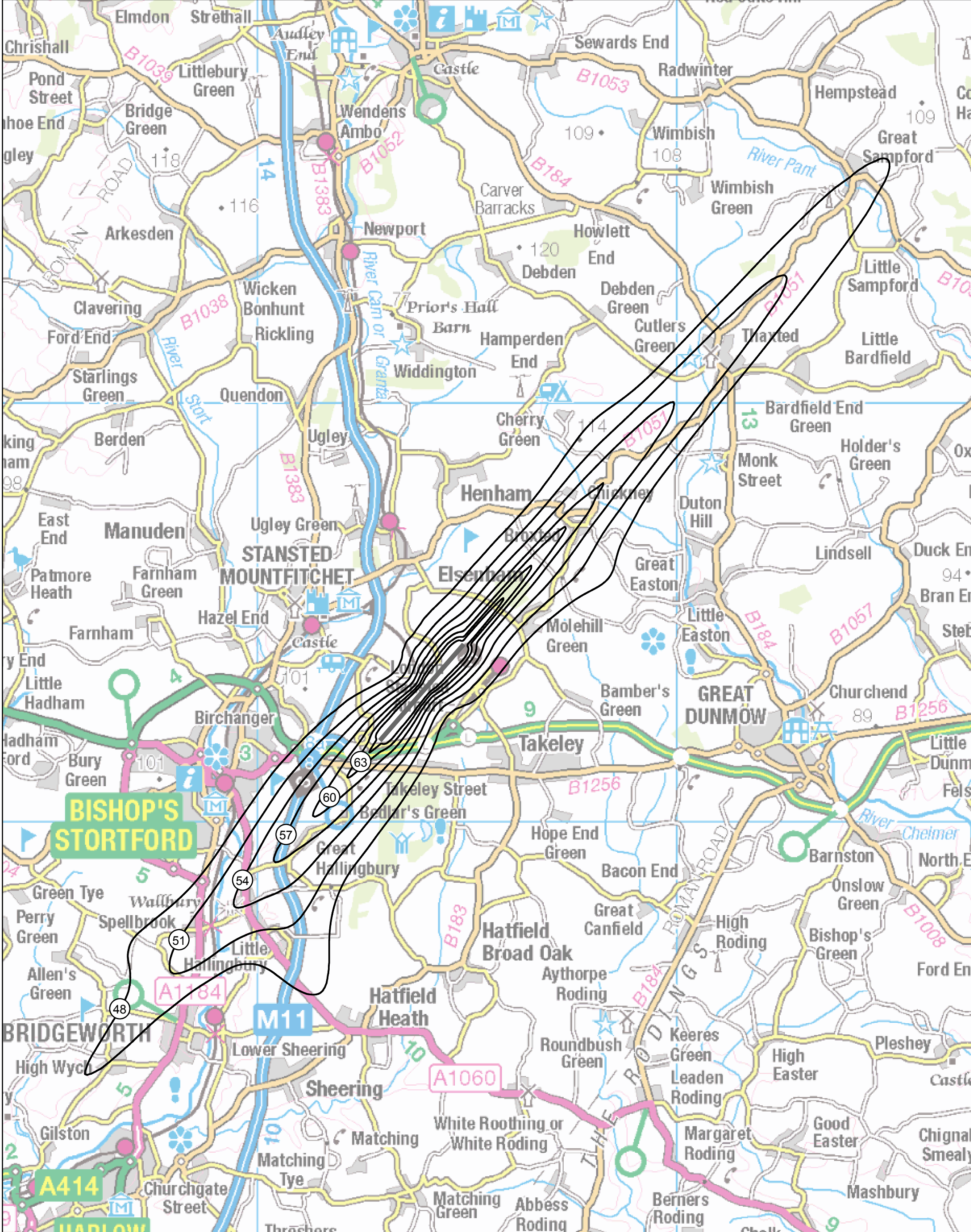
STANSTED AIRPORT Year 2015 Actual Modal Split (73% SW / 27% NE) Average Summer Night (2300-0700 BST) 48-66 dBA Leq Noise Contours
