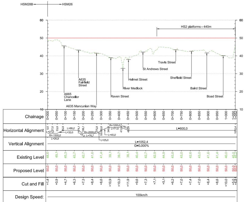
Profile Scale H:1:5,000 V:1:500 @ A1
