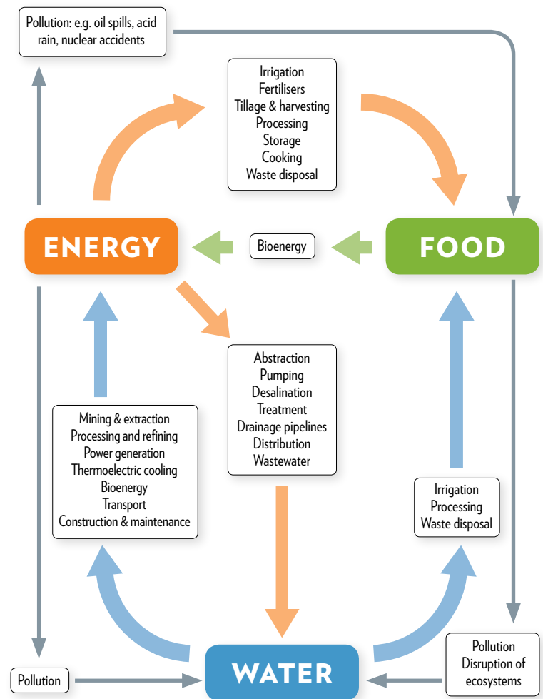
Figure 0-1: An overview of the energy-food-water nexus
