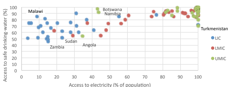
Figure 2-5: Relationship between access to electricity and safe drinking water
