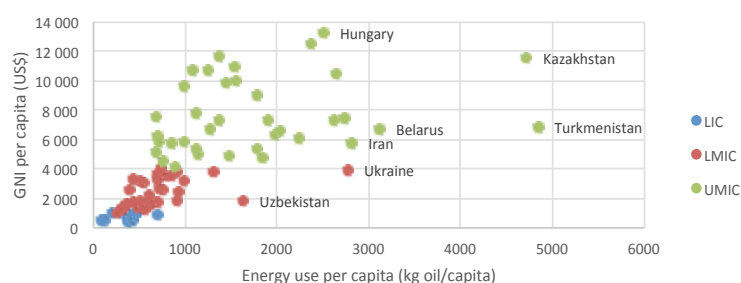
Figure 2-3: Relationship between income and energy use per capita
