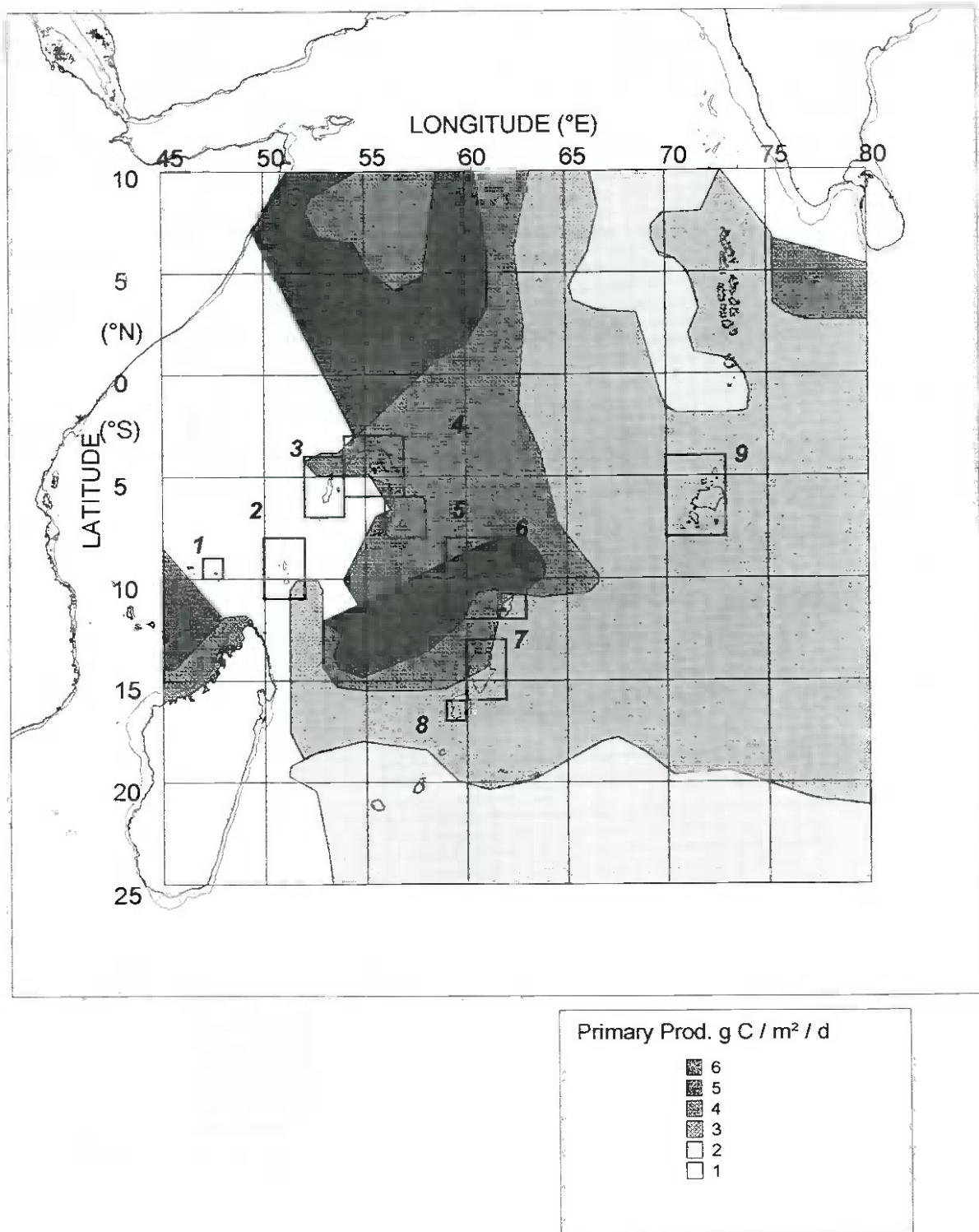
Fig. 7 : The distribution of Primary productivity in the Indian Ocean during the period October - April (after Cushing, 1971)
