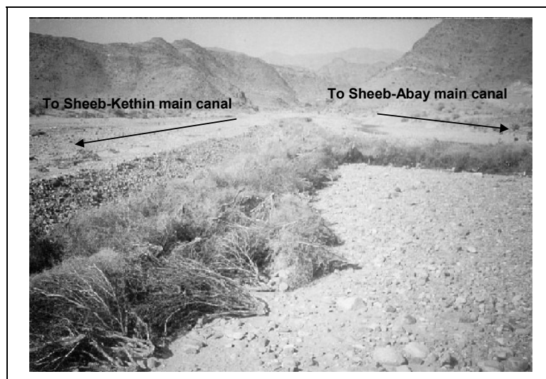
Photograph 1. Wadi Laba indigenous main diversion structure, the Je/wet : ours, 2000
