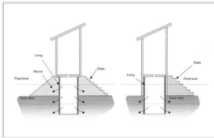
Figure 1: Types of raised pit latrine
