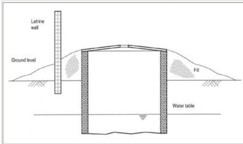
Figure 2: A wide diameter elevated pit latrine
