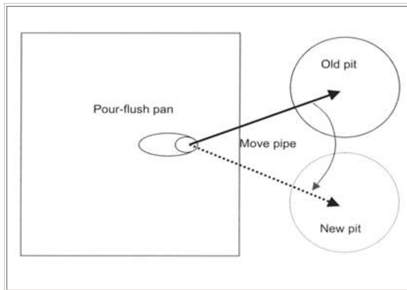
Figure 4: Offset pour-flush latrine with two external pits
