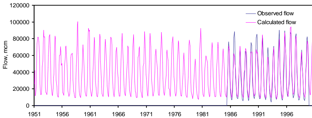
Figure 4.4 Flow in the Mekong at Phnom Penh for 1951 to 2000
