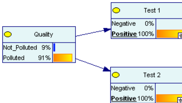
Figure 3.6 Bayesian network for the use of two tests in identifying polluted sites
