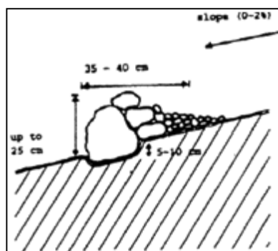
Plate 2.6b: Detail of Stone Bunding
