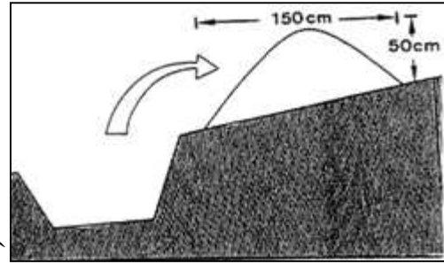
Plate 2.7b: Bund Construction
